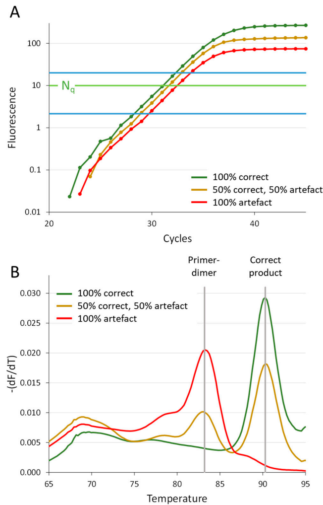
Figure 7. Amplification of correct target and artefact. Different mixtures of intended correct target and primer-dimer artefact were prepared from isolated products and amplified with PCR using the same primer pair for all reactions [11]. (A) Amplification curves showing that the PCR efficiency, determined from the selection of data points in the window of linearity (blue lines [23]), is the same for the correct target, the mixture and the artefact [12]. The difference in plateau level reflects the different lengths of the PCR products. (B) Graph of the negative first derivative of the melting curves ( -dF/dT ) reflects the composition of the mixtures that were amplified. The vertical grey lines indicate the melting temperatures of the correct product (90.3 °C) and the primer-dimer artefact (83.2 °C). The presence of the different products in the three reactions illustrates that the observed C_q values (panel A, N_q ) are correct (green amplification curve), too low (brown curve) or artificial (red curve). The graphs are based on actual amplification data [11].
