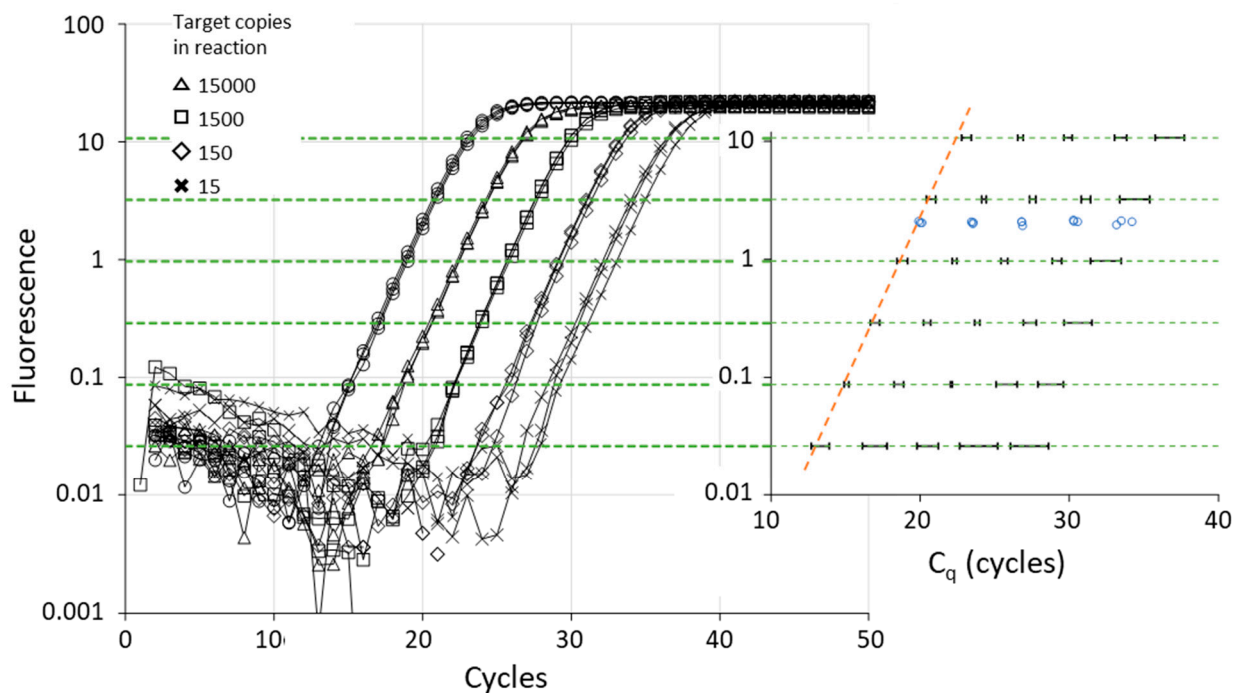
Figure 4. Illustration of relation between threshold level, C_q value and C_q variability. The graph shows the amplification curves of triplicate measurements of a 5-step, 10-fold dilution series. Quantification thresholds (dotted green lines) were placed at six levels between the ground phase noise and the plateau phase. For each of the amplification curves the C_q value was determined. The graph in the inset shows the 95% confidence interval of the observed C_q values (mean \pm 2 \times SD per dilution). The orange dotted line illustrates that when the threshold is set above the exponential phase, the C_q values are higher than expected. The blue dots are the C_q values determined from the SDM (see Section 6.2). The graph is based on actual amplification data.
