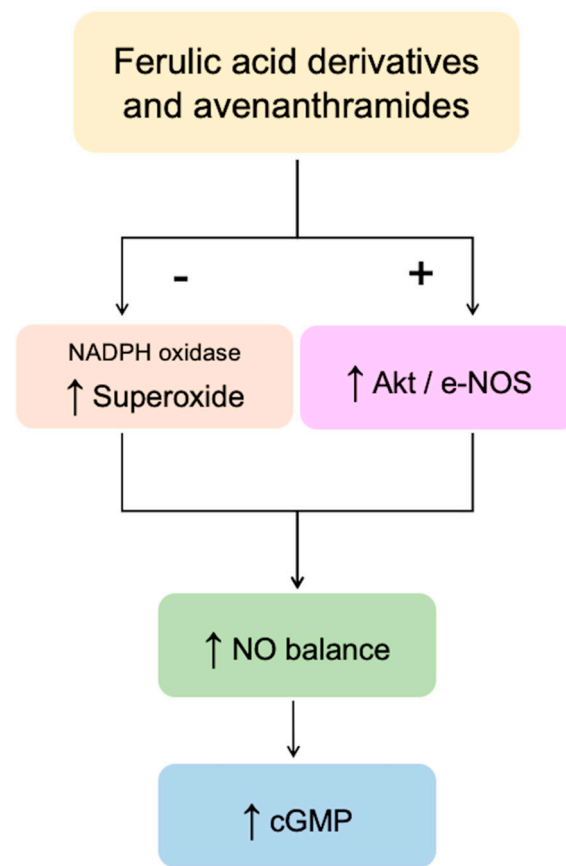
Figure 7. Schematic representation of the mechanisms involved in the modulation of endothelial NO levels by the oat phenolics and metabolites tested in the present study. + = activation; – = inhibition; ↑ = increased.
