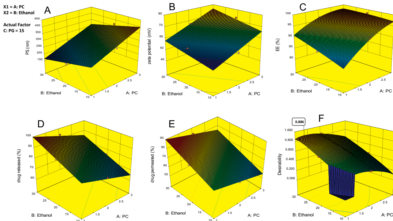
Figure 1 Response surface plot for the effect of independent variables on (A) particle size, (B) ZP, (C) EE%, (D) % drug released over 24 hr, (E) % drug permeated over 24 hr and (F) desirability of the optimized ethosomal RP formula.
