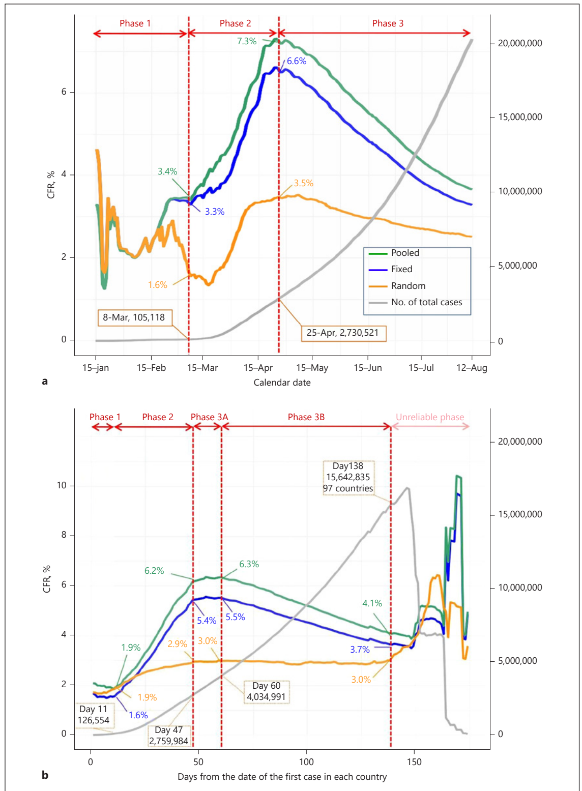
Fig. 3. Timeline of CFR worldwide among countries with COVID-19 reports until August 12, 2020: according to date (a) and according to days (b) since the first confirmed case. COVID-19, coronavirus 2019; CFR, case-fatality rate; Fixed, fixed-effect model; Random, random-effect model; Pooled, calculated CFR based on incidence and mortality data; N, number. Gayda et al. [2].
