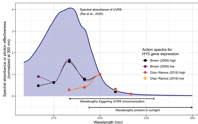
Figure 4 Comparison of published action spectra for UV RESISTANCE LOCUS 8 (UVR8)-mediated expression of the gene ELONGATED HYPOCOTYL 5 ( HY5 ) (Brown et al., 2009; Diaz-Ramos et al., 2018) to the published absorption spectrum of UVR8 (Rai et al., 2020). High and low refer to action spectra computed for different levels of monomerization, as reported in the original publications. All spectra are normalized to one at 300 nm.
