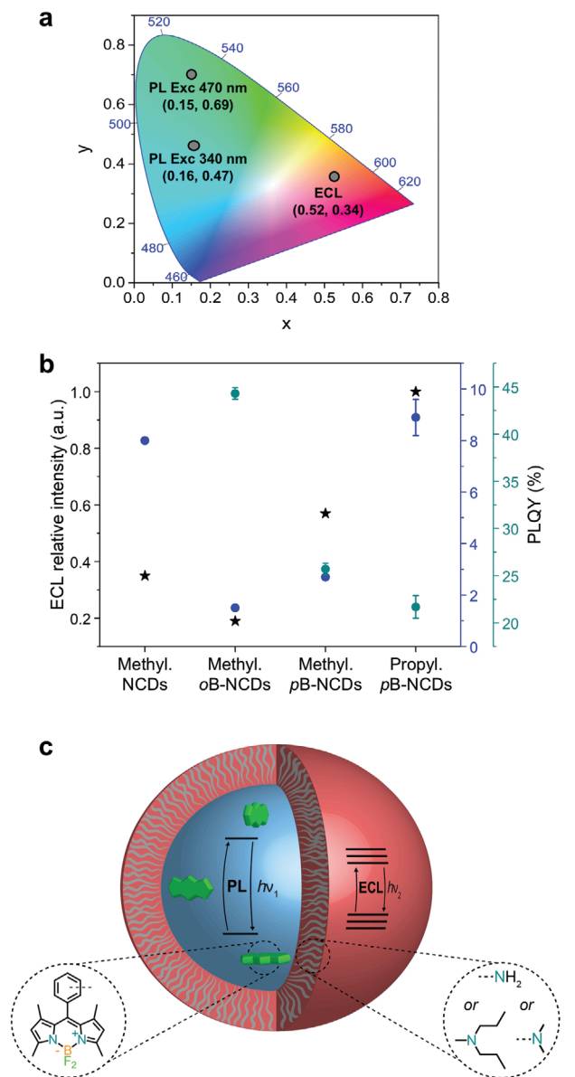
Figure 6. a) 1931 CIE chromaticity diagram showing coordinates from PL (340 nm as excitation wavelength: x = 0.16, y = 0.47 ; 470 nm as excitation wavelength: x = 0.15, y = 0.69 ) and ECL spectra ( x = 0.52, y = 0.34 ) of methylated pB -NCDs. b) ECL relative intensity (black stars), blue PLQY (300 nm as excitation wavelength; blue circles) and green PLQY (466 nm as excitation wavelength; green circles) for methylated NCDs, oB - or pB -NCDs and propylated pB -NCDs. c) Scheme of the core/shell structure of B-NCDs.
