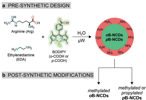
Figure 2. Precursors used for the a) synthesis of oB-NCDs and pB-NCDs and b) post-synthetic modification of the surface amino groups on the surface.
