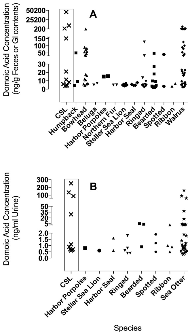
Fig. 2. Domoic acid (DA) concentrations quantified in A) feces and gastrointestinal (GI) contents, and B) urine for all Alaskan species sampled. Domoic acid concentrations detected in 10 California sea lions (CSL) exhibiting signs of DA toxicosis (seizures) are included for reference and shown in the box.
