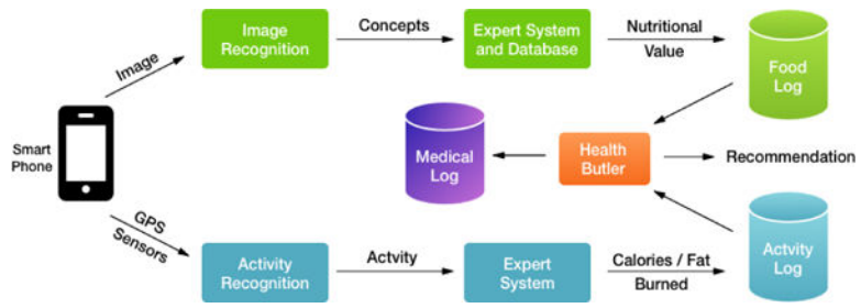
Figure 6: Flow of information in the Health Butler Application, with respect to activity and food event streams.
