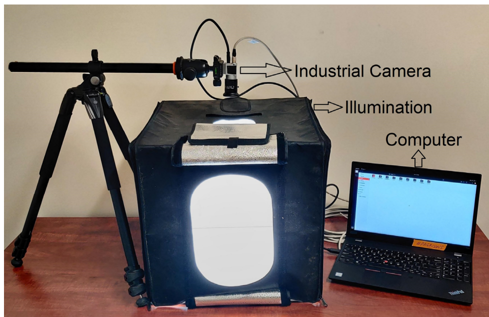
Fig. 1. A typical computer vision system for meat quality non-destructive evaluation applications.
