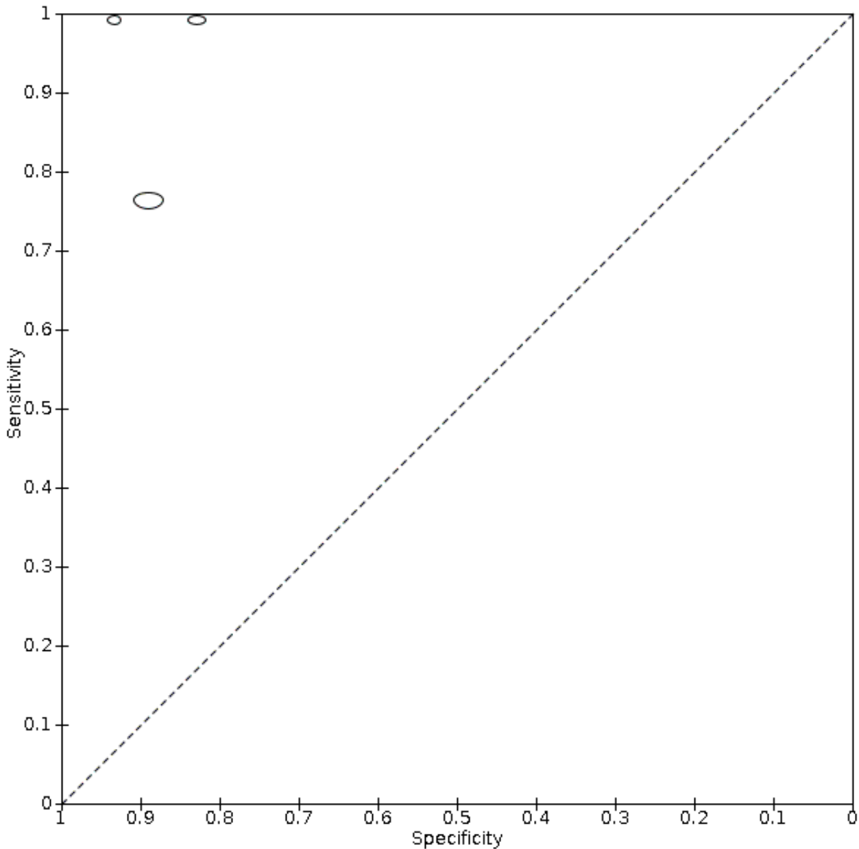
Figure 4. Plot of study sensitivity and specificity in receiver operating curve space.
