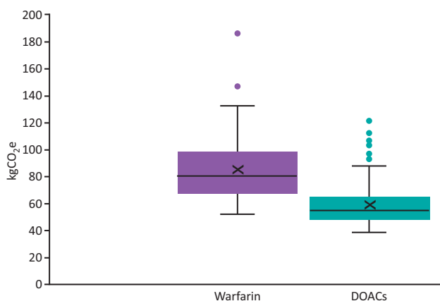
Fig 1. Total kgCO 2 e of the care pathways for warfarin vs DOAC treated patients. DOACs = direct acting oral anticoagulants (and includes the pooled results from the patients receiving rivaroxaban, apixaban and dabigatran).
