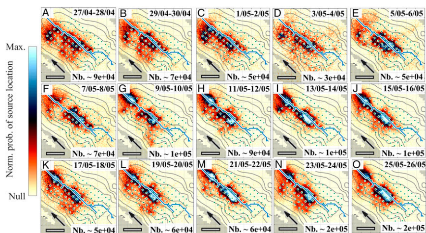
Fig. 3. (A–O) Two-dimensional maps of subglacial water flow source location obtained from MFP. Temporal evolution of the spatial patterns of the source location densities obtained for the 5 \pm 2 Hz frequency range and the [0.07 to 0.16] MFP output range. All of the maps are averaged over 2-d time windows, with the associated number of the sources located shown in the bottom right corner (Nb.). The color scale ranges are normalized for each time window using maximum probability. Contour lines show the 50-m-spaced ice thickness contours, as shown in Fig. 1. The gray shading shows ice-free areas. (Scale bars [Bottom Left], 200 m.) The blue lines show the subglacial waterways, as predicted from the hydraulic potential calculation and as shown in Fig. 1. The black arrows show glacier and subglacial water flow directions. Panel (O) is the characteristic pattern used in Fig. 4 for calculation of the coefficient of determination.
