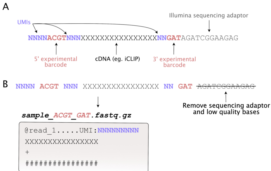
Figure 1. The Ultraplex workflow. A: An example read from a typical iCLIP/ribo-seq library, consisting of twin barcodes, UMIs present at multiple positions, a 3’ sequencing adaptor, and a read derived from a small RNA fragment. B: Flow diagram of the processing of an example read, using combinatorial demultiplexing with single end sequencing data.
