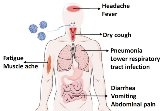
Figure 3 The symptoms of coronavirus infection. Notes: COVID-19 symptoms are similar to other respiratory diseases, such as influenza, SARS, and MERS. However, influenza initiates with cough, whereas COVID-19, like other coronavirus-related diseases initiates with fever. 86 Also, COVID-19 differs from SARS and MERS in the order of gastrointestinal symptoms, where upper gastrointestinal symptoms are seen last after fever and respiratory symptoms. Results supported the use of fever as screen for entry into facilities; however rapid highly sensitive methods for viral confirmation are needed. Illustration reprinted with permission from Chen B, Tian EK, He Betal Overview of lethal human coronaviruses. Signal Transduction and Targeted Therapy . 2020;5(1):1–16. 113 Creative Commons Attribution 4.0 International License ( http://creativecommons.org/licenses/by/4.0/ ).
