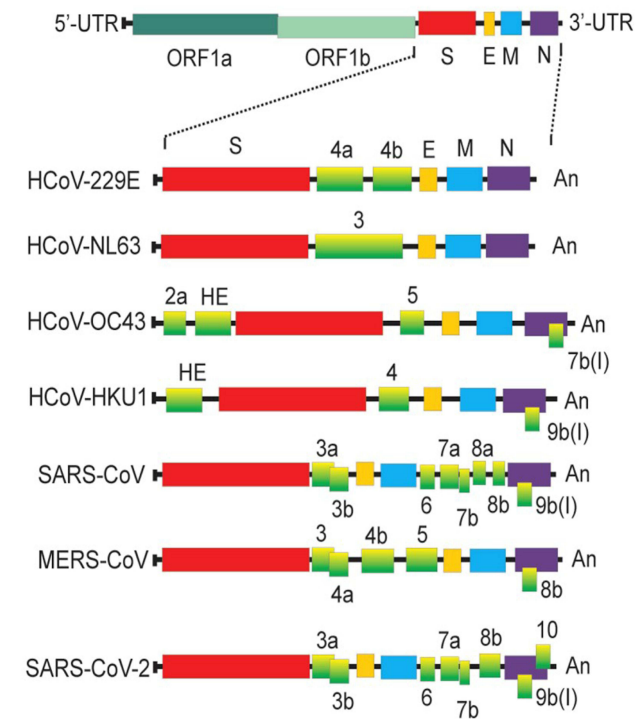
Figure 4 Comparison of different genome structures of coronaviruses. Notes: Reprinted from:Artika IM, Dewantari AK, Wiyatno A. Molecular biology of coronaviruses: current knowledge. Heliyon . 2020;6(8):e04743. 118 Creative Commons CC BY-NC-ND ( http://creativecommons.org/licenses/by-nc-nd/4.0/ ). Abbreviations: UTR, untranslated region; ORF, open reading frame; S, spike protein; E, envelope protein; M, membrane protein; N, nucleocapsid protein.
