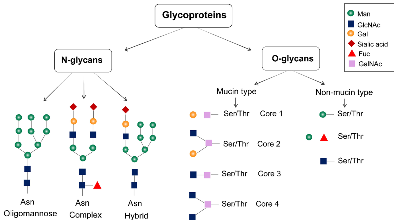
Figure 1 Structure of glycoproteins. Glycoproteins are mainly glycosylated with N-linked and O-linked glycans. N-glycans are attached to the asparagine residues, and they are processed in the Golgi apparatus to yield oligomannose, hybrid, and complex-type N-glycan structures. The mucin-type O-linked glycosylation mainly contains four common O-linked glycan cores. Non-mucin-type O-glycosylations are produced by attaching GlcNAc, mannose, fucose, glucose, galactose, or xylose to the amino acid.
