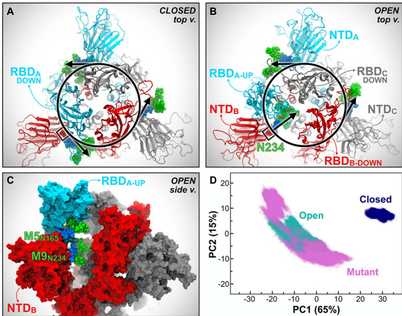
Figure 9 Mutations in the S protein N-glycosylation sites of N234A and N165A show increased instability of RBD-A in the “up” state (A–D). Notes: Reprinted with permission from Casalino LGaieb Z, Goldsmith JA et al Beyond Shielding: The Roles of Glycans in the SARS-CoV-2 Spike Protein. ACS Cent Sci. 2020;6(10):1722–1734. 72 Copyright © 2020 American Chemical Society. Further permissions related to the material excerpted should be directed to the ACS. Available from: https://pubs.acs.org/doi/10.1021/acscentsci.0c01056 .
