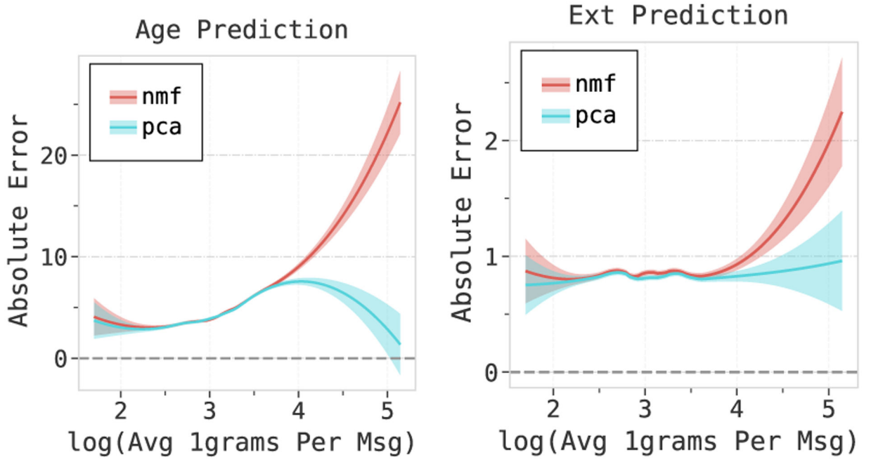
Figure 2: Comparison of the absolute error of NMF and PCA with the average number of 1 grams per message. While both the models appear to perform very similar when the texts are small or average sized, PCA is better at handling longer texts. The errors diverge when the length of the texts increases.
