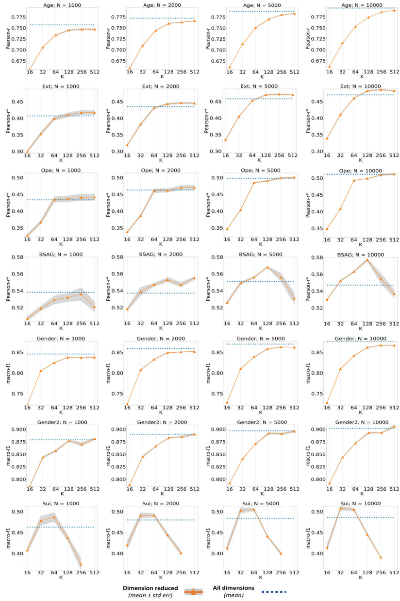
Figure A2: Performance recorded for reduced dimensions for all tasks at higher N_{ta} values ( 1000). Reduction continues to help in performing the best in personality and mental-health tasks. The ' f_{kp} ' is observed to be shifting to a higher value, due to the rise in performance of no reduction and the reduction of standard error.
