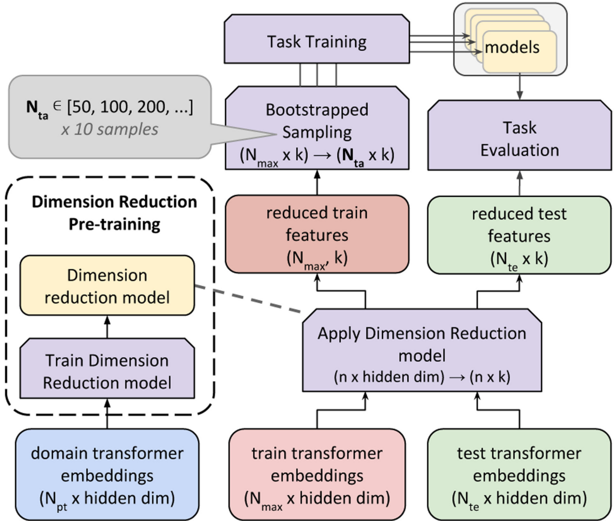
Figure A1: Depiction of Dimension Reduction method -
