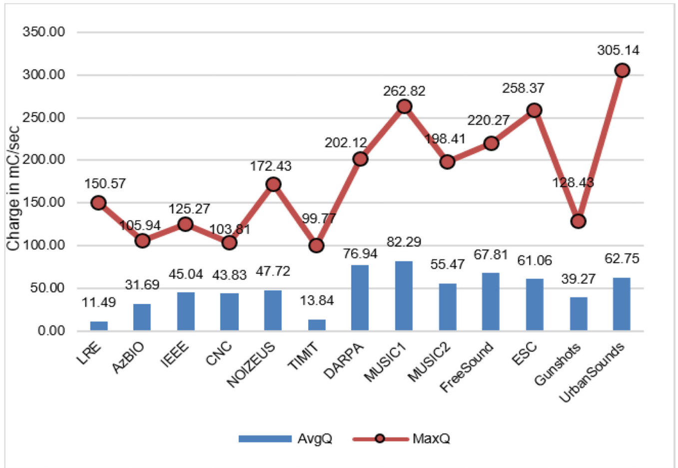
Figure 5: Performance of charge/sec against database
