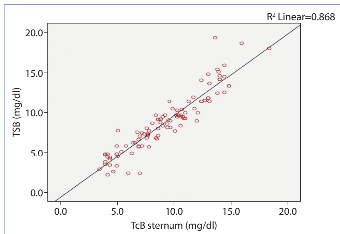
Figure 2. Linear regression analysis between TSB and TcB sternum measurements ( R^2=0.87 ).
