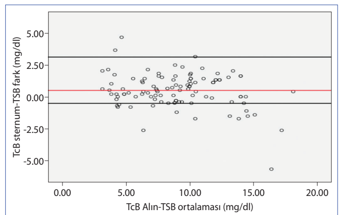
Figure 4. Bland-Altman analysis between TSB and TcB sternum measurement methods (average difference: 0.49 \pm 1.32 , %95 CI: [-2.1] – [3.07] , upper limit: 3.07, lower limit: -2.1 ).
