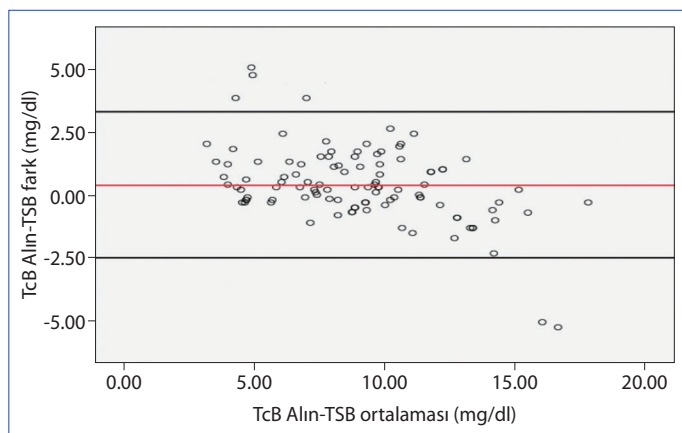
Figure 3. Bland-Altman analysis between TSB and TcB forehead measurement methods (average difference: 0.39 \pm 1.46 , 95% CI: [-2.47] – [3.26] , upper limit: 3.26, lower limit: -2.47 ).
