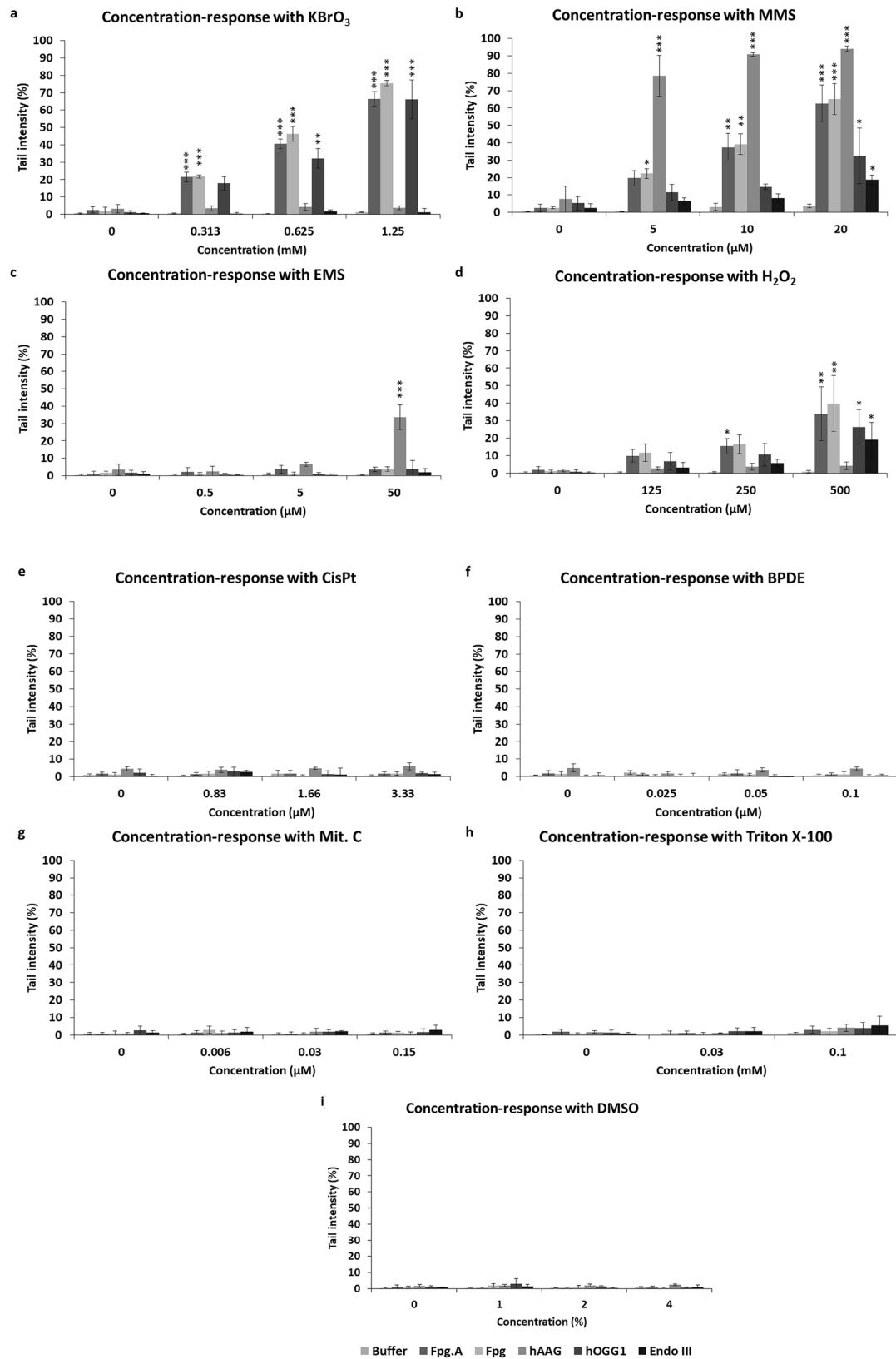
Fig. 1 Enzyme-modified comet assay. Results (tail intensity) obtained in TK-6 cells after 3 h of treatment with different compounds (a–i) are expressed as SB and ALS (in “Buffer”) or net enzyme-sensitive
