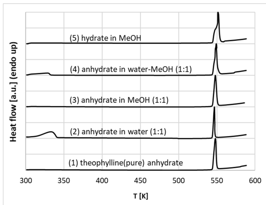
Figure 5. Thermograms of the products of milling of pure commercial anhydrous theophylline (1), anhydrate co-grinded with equimolar amounts of neat water (2), neat methanol (3), aqueous unimolar mixture with methanol (4) and monohydrate co-grinded with methanol (5).
