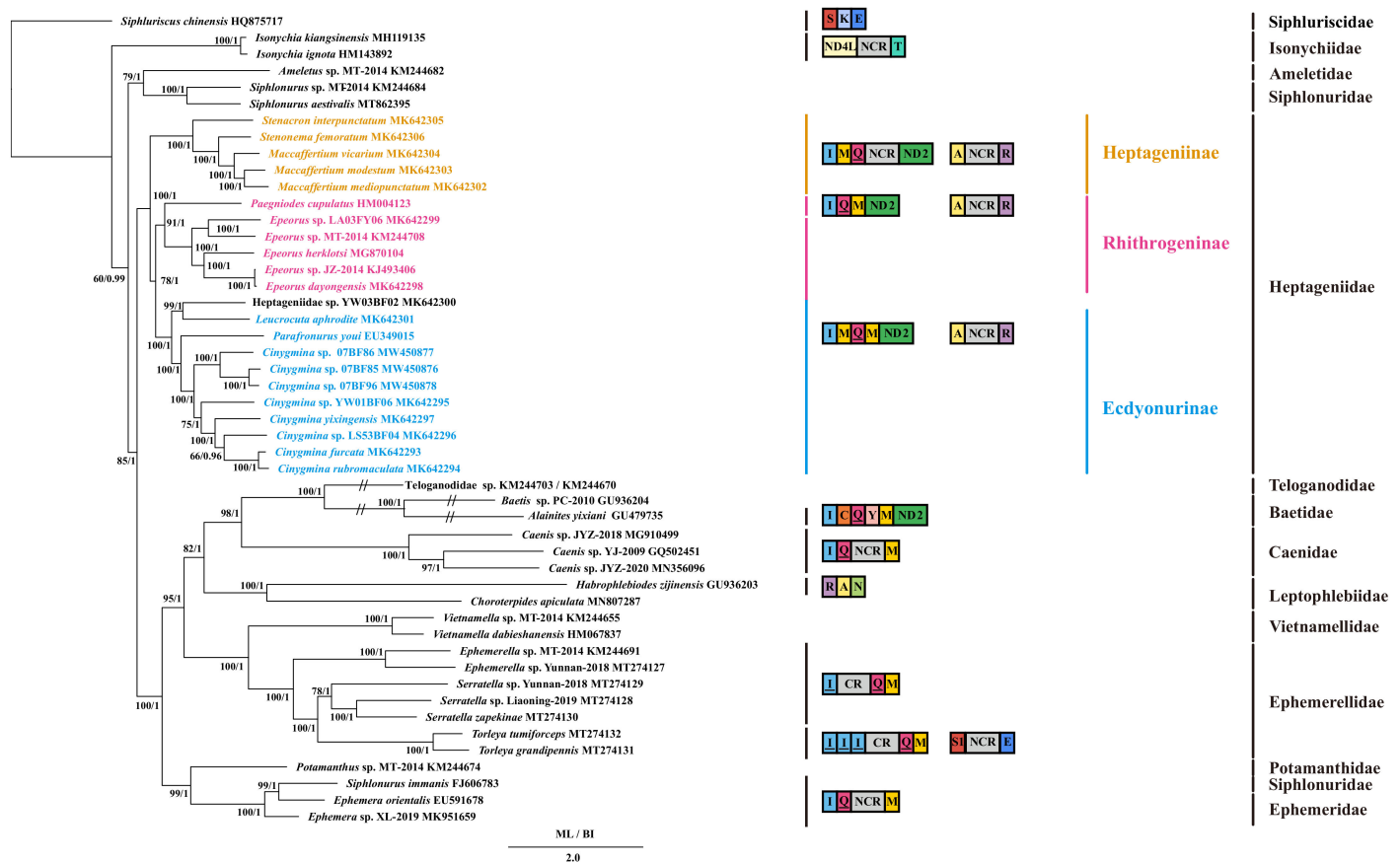
Figure 3. Phylogenetic tree of the relationships among 49 species of Ephemeroptera according to the nucleotide dataset of the 13 mitochondrial PCGs. Siphuriscus chinensis was used as the outgroup. The numbers above branches specify bootstrap percentages from ML (left) and posterior probabilities as determined from BI (right). The GenBank accession numbers of all species are shown in the figure. Box images on the right show gene rearrangements and the location of the NCR for the various mayfly species. Genes encoded by the minority strand are underlined, and those without underline are encoded by the majority strand. Different colored boxes represent different genes. The remaining genes and gene orders that were identical to the ancestral insect are left out. Gene sizes are not drawn to scale. The asterisks (*) by Siphonuridae on the far-right side denote the separation of these sequences.
