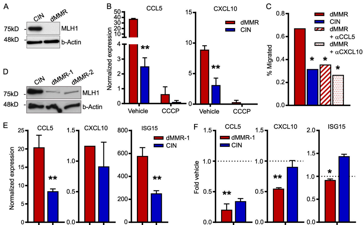
Figure 7. Loss of DNA mismatch repair in primary mouse and CRC patient organoids up-regulates chemokine production and type I IFN signaling. (A) Baseline protein expression from primary mouse CRC organoids. CRC was induced by 10 weekly injections of 10 \mu\text{g}/\text{kg} azoxymethane followed by another 10 wk without treatment. Mlh1 was stably knocked down by lentiviral transduction with shRNA and hygromycin selection to establish dMMR organoids. Scrambled shRNA-transduced organoids were used as CIN controls. n = 4 repeats. (B) Reduced expression of ISGs following 24 h incubation of the dMMR and CIN organoids with 10 \mu\text{M} of the cGAS/STING inhibitor CCCP. n = 3 repeats. dMMR versus CIN: **, P \leq 0.01 . (C) CD8 + T cell migration toward supernatant conditioned for 24 h by established dMMR or CIN organoids. dMMR versus indicated bar. *, P \leq 0.05 . (D and E) Baseline protein (D) and RNA (E) expression in organoids established from CRC patients. dMMR organoids were generated by stably knocking down MLH1 as in A with the appropriate shRNA and Scramble CIN control. dMMR versus CIN: **, P \leq 0.01 . (F) Inhibition of chemokine and ISG expression by treatment of human CRC organoids for 24 h with 10 \mu\text{M} CCCP. n = 2 patients, three repeats each. Vehicle versus *, P \leq 0.05 ; **, P \leq 0.01 .
