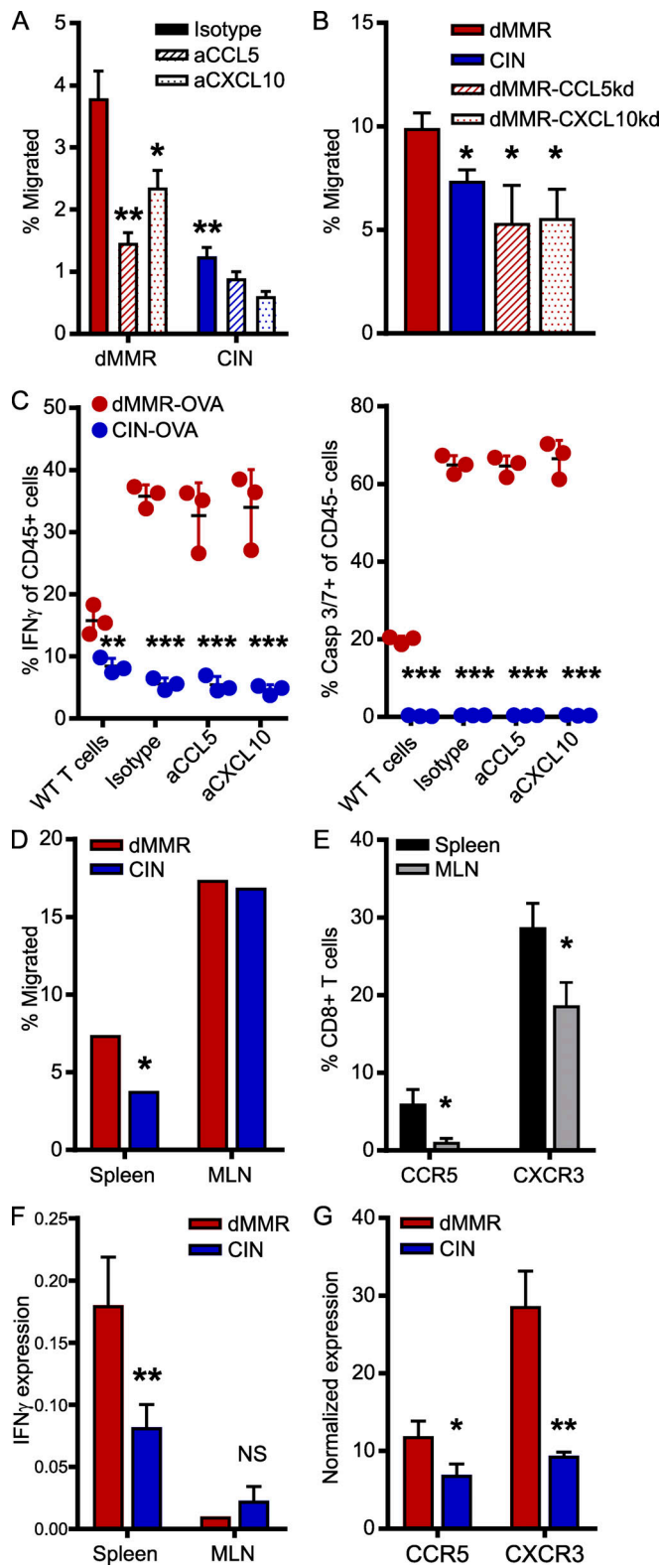
Figure 2. CCL5 and CXCL10 expression is essential for the recruitment and activation of systemic CD8+ T cells by dMMR CRCs. (A) CD8+ T cell migration through a Matrigel-coated 5.0- \mu m Transwell insert toward supernatant conditioned for 24 h by dMMR or CIN MC38 CRCs. Anti-CCL5, CXCL10, or isotype control antibodies were added at 2.0 \mu g/ml 30 min before T cells were added. Migrated cells were quantified after 2 h by flow cytometry. n = 5 repeats. (B) CD8+ T cell migration toward supernatant
