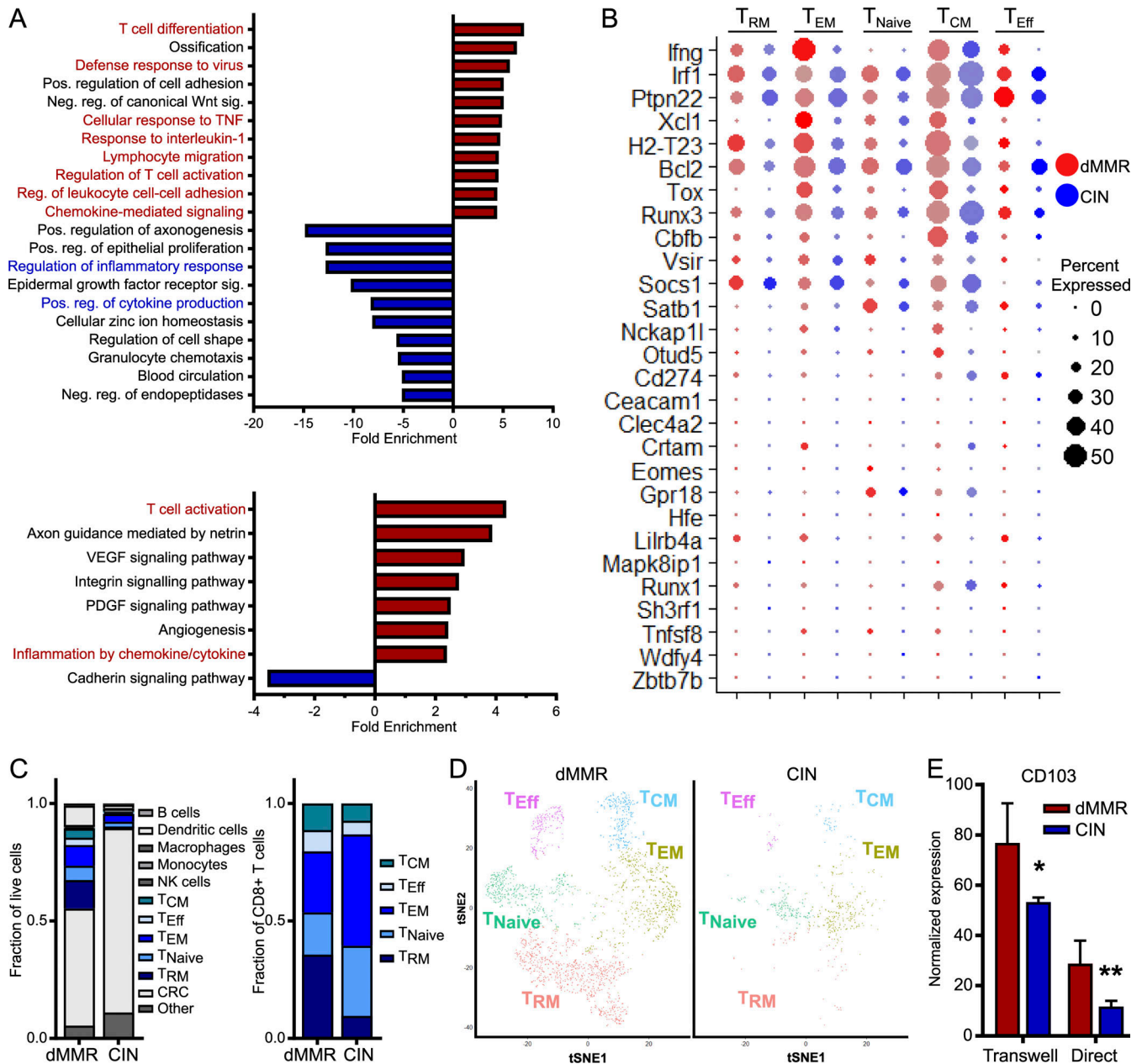
Figure 4. Orthotopic dMMR CRCs up-regulate TRM markers on infiltrating systemic CD8 + T cells. scRNAseq was performed on orthotopically grown dMMR and CIN CRCs. Five mice were pooled from each CRC type. (A) GO enrichment analysis of the most enriched biological processes (top) and signaling pathways (bottom) for CD8 + T cells in orthotopic dMMR compared with CIN CRCs. (B) Expression of genes in the “CD8 T Cell Activation” GO term list. Size of the dot represents percent of cells and color intensity represents expression level. (C) Proportion of cell types identified by scRNAseq within the tumor microenvironment of orthotopic dMMR and CIN CRC (left) and within the CD8 + T cell subsets (right). T Naive , naive T cells; T EM , effector memory T cells; T Eff , effector T cells; T CM , central memory T cells. (D) tSNE plots of CD8 + T cell subsets identified by scRNAseq in orthotopic dMMR and CIN CRCs. (E) Induction of CD103 in CD8 + T cells by dMMR and CIN CRCs was measured by qPCR after coculturing cells directly or separated by a 0.4- \mu m Transwell filter for 24 h. Representative data from n = 3 repeats. dMMR versus CIN: *, P \leq 0.05 ; **, P \leq 0.01 . Neg., negative; Pos., positive; Reg., regulation; Sig., signaling.
