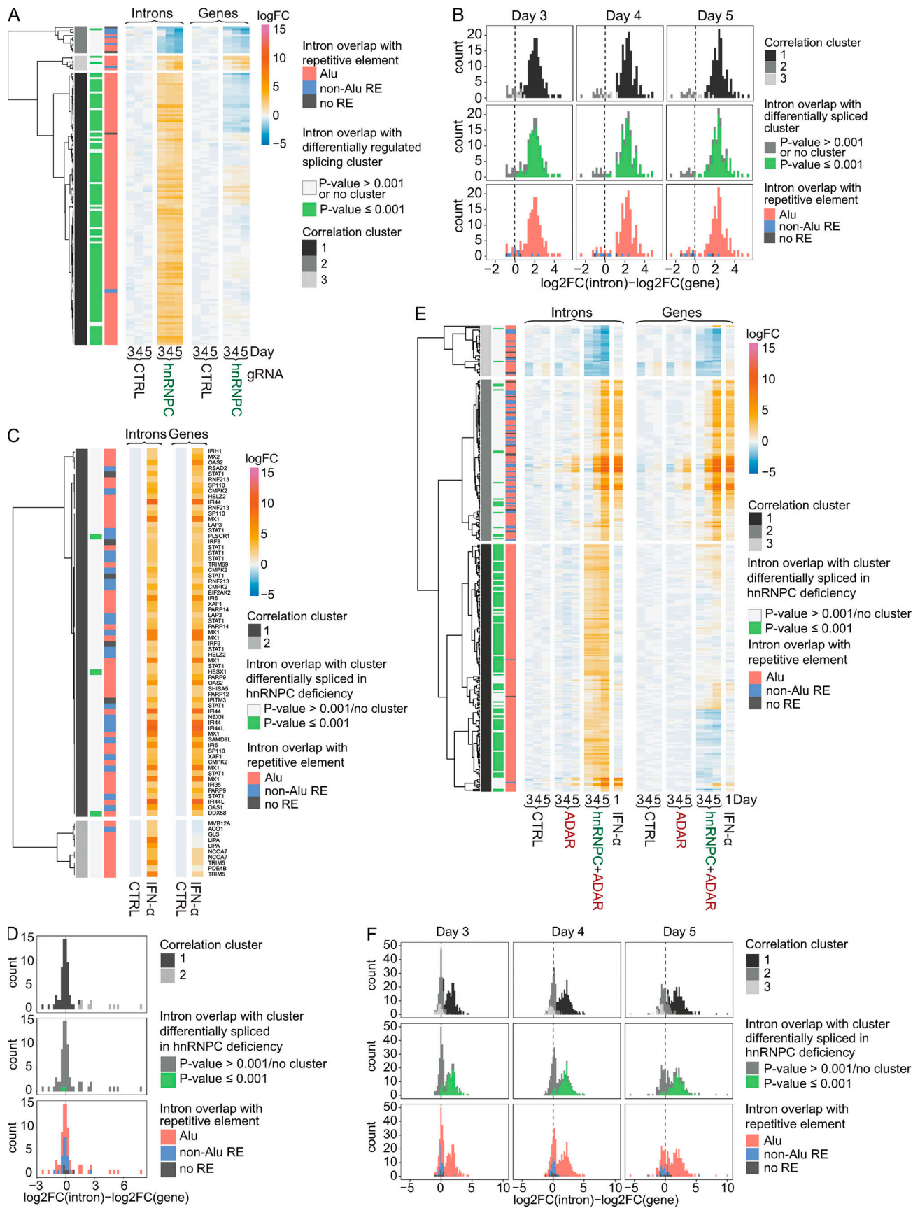
Figure 5. Splicing-dependent intron dysregulation is independent of gene expression. (A, C, and E) Heatmap of expression of differentially regulated introns (left, fold change \geq 4 , FDR-adjusted P value \leq 0.01 in any per-day pairwise comparison) and their respective genes (right) in nontarget control (CTRL)
