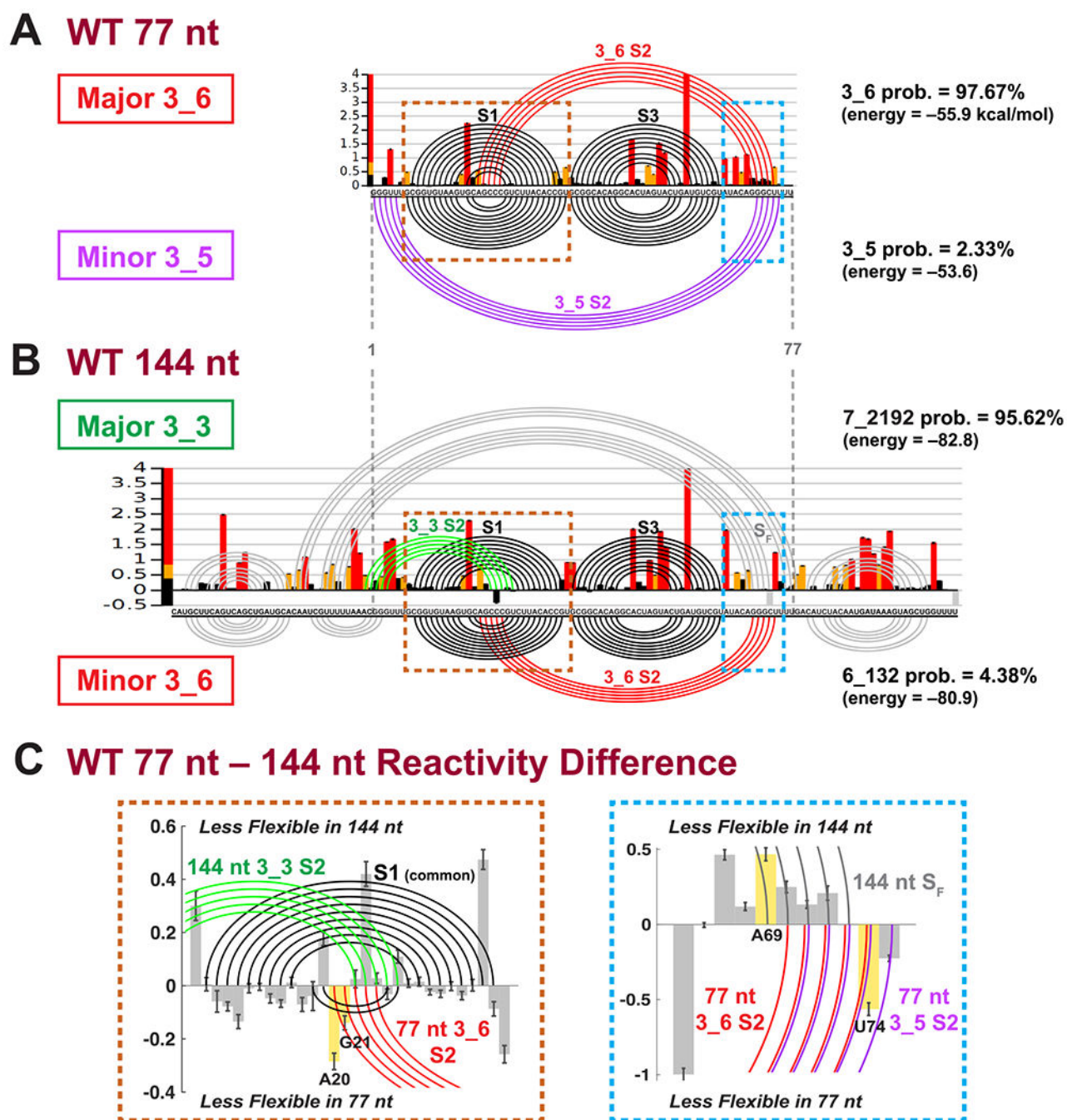
Figure 4. SHAPE reactivity analysis for SARS-CoV-2 frameshifting element for 77 and 144 nt (Replicate 1). (A) The SHAPE reactivity for the 77 nt construct is plotted by bars, with red/yellow/black representing high/medium/low reactivity. The arc plot at top shows the dominant 3_6 pseudoknot predicted by the ShapeKnots energy landscape (98% of conformational space), and at bottom is the minor 3_5 (2% of landscape). Stems are labeled, and the Gibbs free energy (kcal/mol) and Boltzmann distribution probabilities are given. (B) SHAPE reactivity and ShapeKnots predictions for 144 nt construct. (C)
