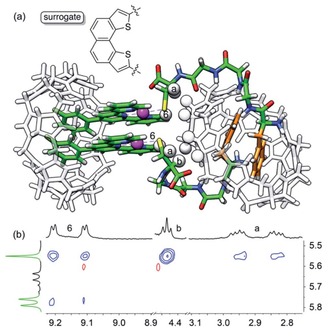
Fig. 5 (a) Most stable structure of pendant necklace \text{CB}[8]^{\text{Pt}}_2 \cdot 12 \cdot \text{CB}[8]^{\text{Phe}}_{\text{HT}} optimized at the B97-3c/def2-mTZVP level. Hydrogen atoms interacting through space are highlighted with white spheres. (b) ^1\text{H}-^1\text{H} NOESY spectrum in \text{D}_2\text{O} at 25 °C of assembly \text{CB}[8]^{\text{Pt}}_2 \cdot \text{CB}[8]^{\text{Phe}}_{\text{HT}} where cross-peaks of hydrogens H6, \text{H}^a and \text{H}^b with \text{CB}[8]^{\text{Phe}} hydrogens are observed; signals pertaining to \text{CB}[8]^{\text{Phe}} appear in green.
