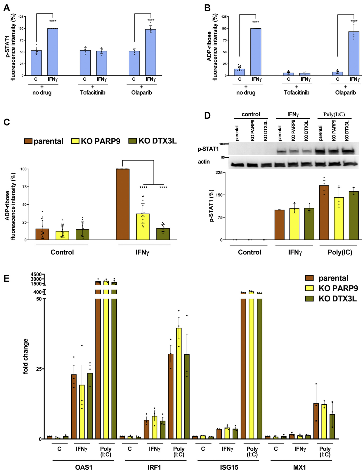
Figure 4. IFN-inducible PARP9 and DTX3L are required for IFN-induced ADP-ribosylation. A , quantification of nuclear STAT1 phospho-Y701 immunofluorescence signal intensity in A549 cells 24 h after treatment with vehicle control or 100 U/ml IFN \gamma , with or without 10 \mu M tofacitinib or 10 \mu M olaparib, as indicated. Mean \pm SEM ( n = 6 , from three separate experiments), **** p < 0.0001 . B , quantification of ADP-ribose immunofluorescence signal intensity in A549 cells 24 h after treatment with vehicle control or 100 U/ml IFN \gamma , with or without 10 \mu M tofacitinib or 10 \mu M olaparib, as indicated. Mean \pm SEM ( n = 6-10 , from three separate experiments), **** p < 0.0001 . C , quantification of ADP-ribose immunofluorescence signal intensity in WT, PARP9 or DTX3L KO RPE1-hTERT cells 24 h after treatment with vehicle control or 100 U/ml IFN \gamma . Mean \pm SEM ( n = 11-17 , from four separate experiments), **** p < 0.0001 . D , representative image ( top ) and quantification ( bottom ) of immunoblot analyses for STAT1 phospho-Y701 and actin loading control in WT, PARP9 KO, or DTX3L KO RPE1-hTERT cells 24 h after treatment with either vehicle control, 100 U/ml IFN \gamma , or transfection
