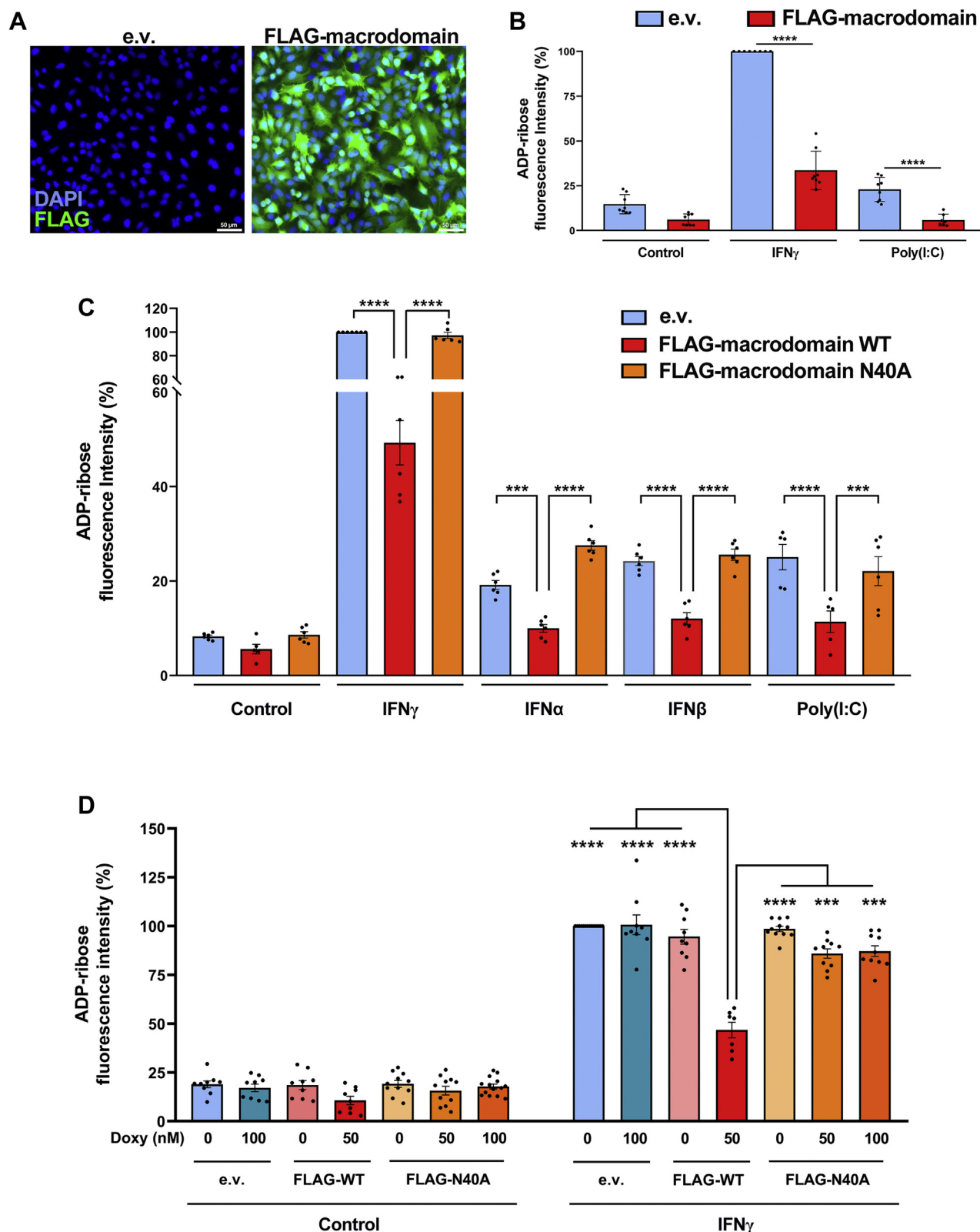
Figure 2. Ectopic expression of the Nsp3 macrodomain reverses IFN-induced ADP-ribosylation. A , representative images of anti-FLAG immunofluorescence staining (green) and DAPI staining (blue) in A549 cells transfected either with an empty vector control (left) or with a lentiviral construct constitutively expressing FLAG-tagged SARS-CoV-2 Nsp3 macrodomain (right). Scale bars = 20 \mu m. B , quantification of ADP-ribose immunofluorescence signal intensity in A549 cells transfected either with empty vector control (e.v.) or with a lentiviral construct for constitutive expression of FLAG-tagged macrodomain 24 h after treatment with vehicle control, 100 U/ml IFN \gamma or transfection with 0.1 \mu g/ml poly(I:C). Mean \pm SEM (n = 8, from three separate experiments), ****p < 0.0001. C , quantification of ADP-ribose immunofluorescence signal intensity in A549 cells transfected either with empty vector control (e.v.) or with lentiviral constructs for constitutive expression of either WT macrodomain or catalytically dead N40A mutant, after 24 h treatment with 1000 U/ml IFN \alpha , 1000 U/ml IFN \beta , 100 U/ml IFN \gamma , transfected with 0.1 \mu g/ml poly(I:C) or vehicle control. For FLAG-macrodomain-expressing samples, cells were gated
