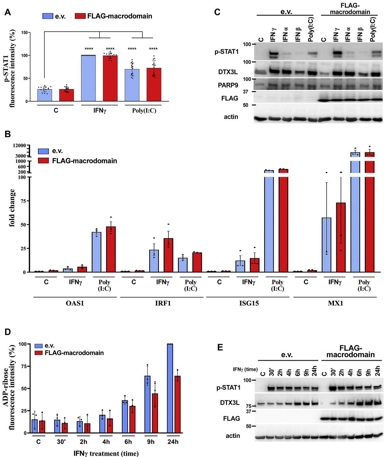
Figure 5. Nsp3 macrodomain expression has no effect on IFN signaling. A , quantification of nuclear STAT1 phospho-Y701 immunofluorescence signal intensity in A549 cells transduced either with empty vector control (e.v.) or with a lentiviral construct for constitutive expression of FLAG-tagged macrodomain, 24 h after treatment with vehicle control, 100 U/ml IFN \gamma , or transfection with 0.1 \mu g/ml poly(I:C). Mean \pm SEM ( n = 14 , from three separate experiments), **** p < 0.0001 . B , relative levels of mRNA for OAS1, IRF1, ISG15, and Mx1 genes determined by RT-qPCR in A549 cells transduced either with empty vector control (e.v.) or with a lentiviral construct for constitutive expression of FLAG-tagged macrodomain, 24 h after treatment with vehicle control, 100 U/ml IFN \gamma , or transfection with 0.1 \mu g/ml poly(I:C), normalized to respective vehicle-treated empty vector control cells. Mean \pm SEM ( n = 3 ). C , representative image of immunoblot analyses for STAT1 phospho-Y701, DTX3L, PARP9, FLAG, and actin loading control in A549 cells transduced either with empty vector control (e.v.) or with a lentiviral construct for constitutive expression of FLAG-tagged macrodomain, 24 h after treatment with vehicle control,
