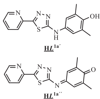
Chart 2. Oxidation Products of HL 1 and HL 2 and Copper(II) Complexes with Oxidized Ligands a
