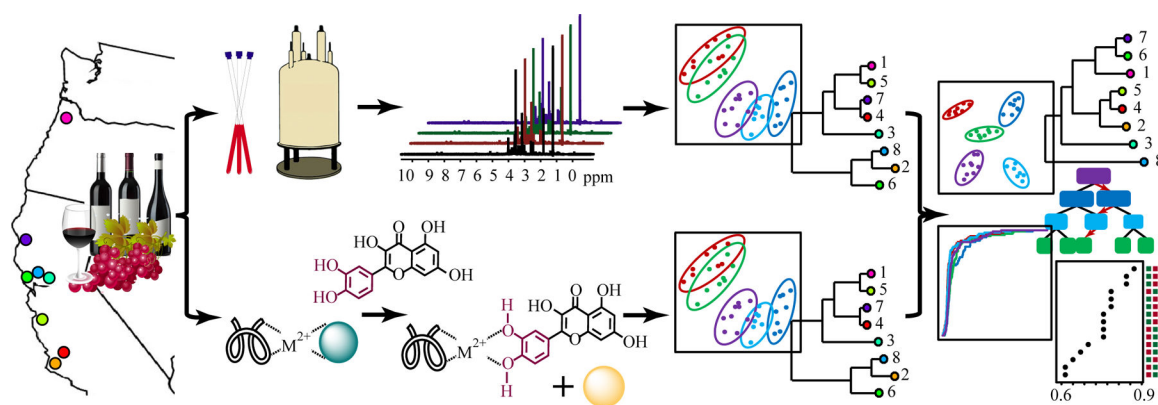
Figure 1. Schematic Representation of Pinot noir Combined Wine Classification. The combined experimental approach utilized NMR spectroscopy and DS array of phenolics ( e.g. , flavonoids, tannins). The analytical techniques were combined to discriminate fifteen Pinot noir wines from nine AVAs along the coast of California and Oregon. A combination of multivariate and univariate statistical methods was used to produce a classification model that differentiate wines based on vineyard, AVA region or vintage.
