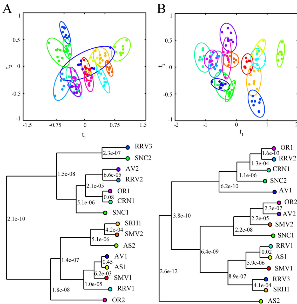
Figure 3. Vineyard Multivariate Scores Plots. LDA-MB-PCA scores plots and associated dendrograms generated from the combined NMR spectroscopy and DS array datasets from the (A) 2015 ( R^2 0.78, Q^2 0.53) and (B) 2016 ( R^2 0.67, Q^2 0.54) wine samples. LDA-MB-PCA scores plots and dendrograms are displayed with color-coded groups labels, symbols and ellipses as defined in Figure 2. Ellipses represent the 95% confidence interval from a normal distribution. Each node of the dendrogram is labeled with a p-value based on Mahalanobis distances between the groups. LDA models were generated from the first four components of the MB-PCA model.
