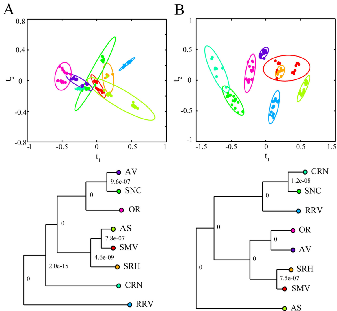
Figure 4. AVA Region Multivariate Scores Plots. LDA-PCA scores plots and associated dendrogram models generated from the NMR spectroscopy region datasets from the (A) 2015 ( R^2 0.79, Q^2 0.74) and (B) 2016 ( R^2 0.75, Q^2 0.70) wine samples. LDA-PCA scores plots and dendrograms are displayed with color-coded groups labels, symbols and ellipses as defined in Figure 2. Ellipses represent the 95% confidence interval from a normal distribution. Each node of the dendrogram is labeled with a p-value based on Mahalanobis distances between the groups. LDA models were generated from the first four components of the PCA model.
