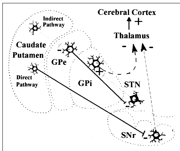
FIG 4. The indirect pathway and the direct pathway in the circuitry of the basal ganglia. Minus sign indicates postsynaptic inhibition; plus sign indicates postsynaptic excitation. In our hypothesis of the mechanism for generating ballism, dashed lines indicate hypoactivity of the pathway and solid lines indicate hyperactivity of the pathway. Lesions in the caudate putamen (indirect pathway) or subthalamic nucleus and hyperactivity in the caudate putamen (direct pathway) can result in thalamic disinhibition. GPe , external segment of globus pallidus; GPi , internal segment of globus pallidus; SNr , substantia nigra pars reticulata; STN , subthalamic nucleus.
