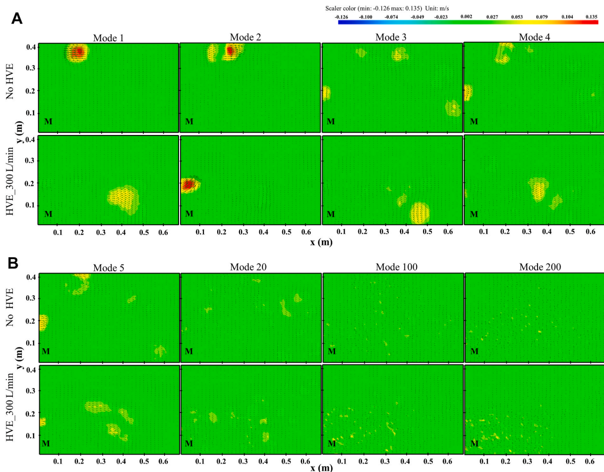
Fig. 5. Typical POD modes of the fluctuation flow field under whether the cooperation of the HVE (300 L/min). The coordinates of the mannequin’s mouth are (0.05 m, 0.05 m), referred to by “M”.
