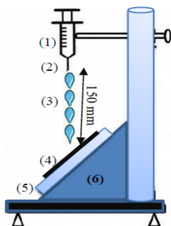
Figure 2. Schematic diagram for the water repellency spray tester containing (1) syringe, (2) jet nozzle, (3) water drop, (4) fabric sample, (5) support inclined at 45^\circ , and (6) holder.
