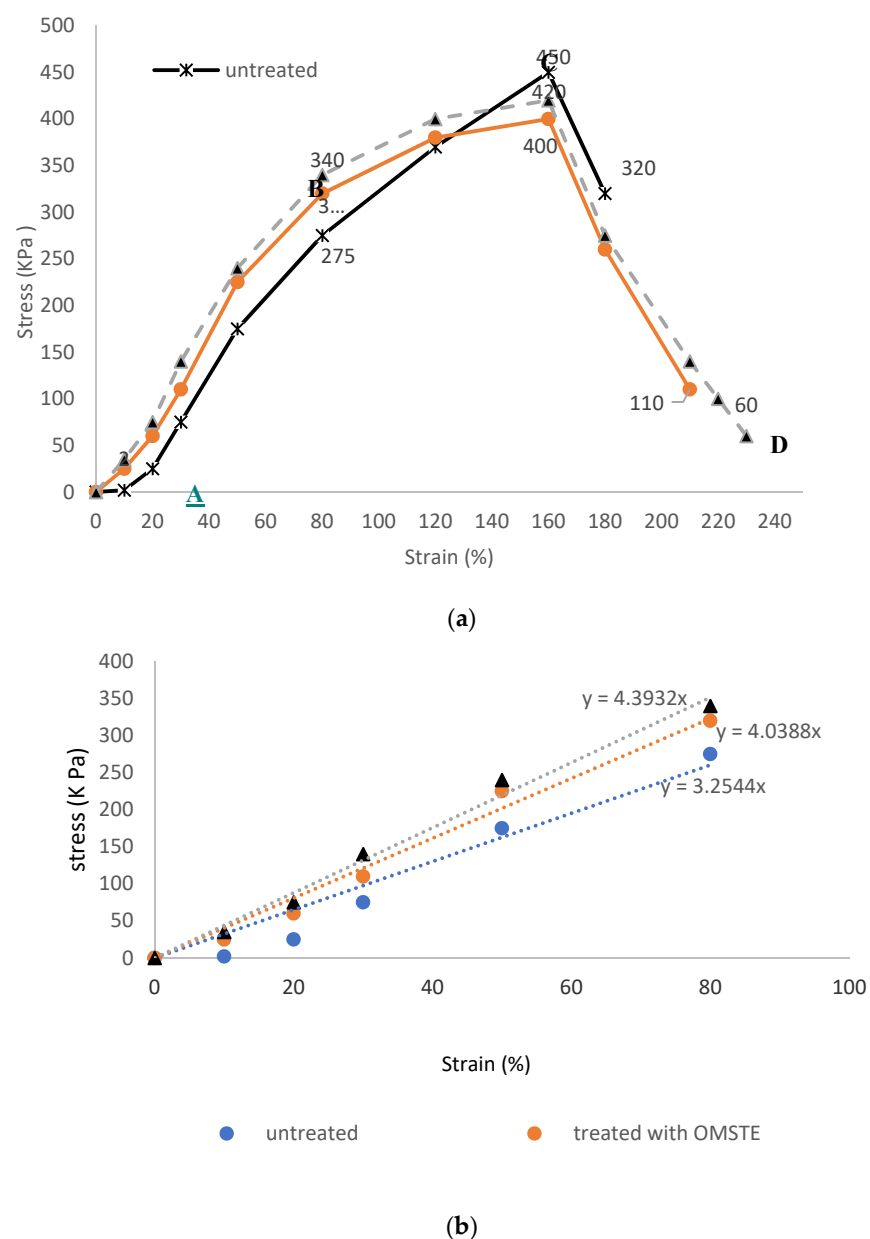
Figure 12. (a) The relation between stress \sigma (KPa) as a function of the strain \epsilon (%) for untreated and treated samples with DC plasma reactors OMTSE and OMSE. (b) The elastic region AB, exhibiting straight lines, with the slope represents Young's modulus (stiffness).
