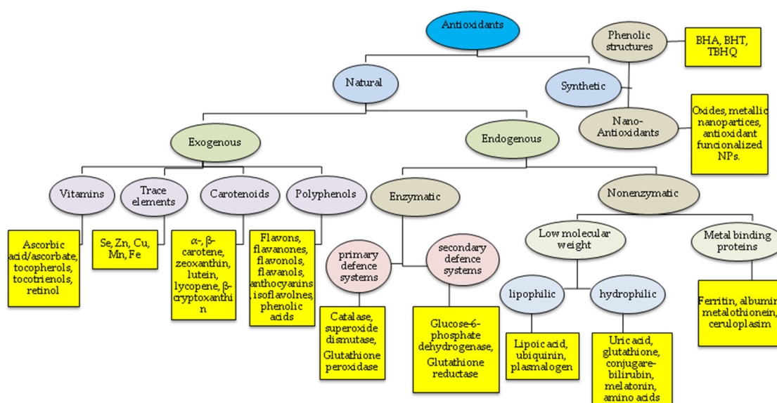
Figure 1. Antioxidants classification.
