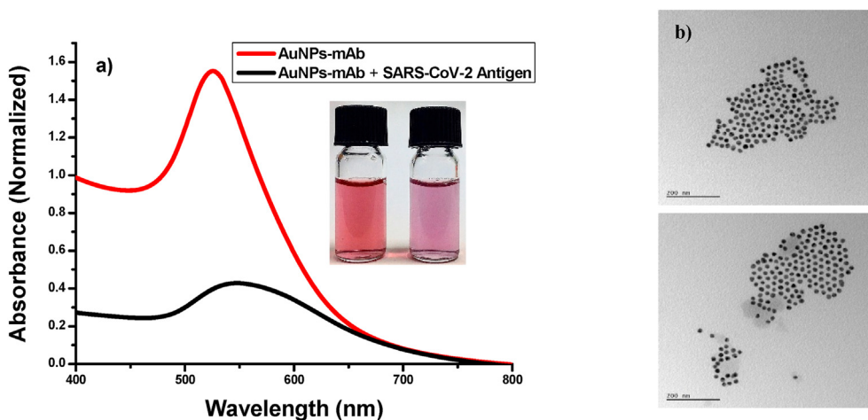
Fig. 3. (a) Absorption spectra of AuNPs-mAb in the absence (red line) and presence (black line) of 2 \mu\text{g}/\text{mL} of the SARS-CoV-2 spike antigen. (b) TEM images of AuNPs-mAb after incubation with the SARS-CoV-2 spike antigen. Scale bar: 200 nm. (For interpretation of the references to color in this figure legend, the reader is referred to the Web version of this article.)
