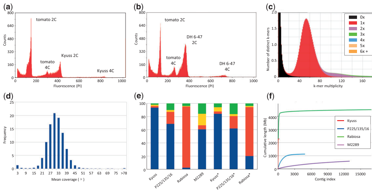
Fig. 1. —Features of the Kyuss genome and assembly. (a) Flow cytometry trace of Kyuss nuclei showing the occurrence of peaks at the same position as in the diploid parent (b) when compared with the tomato external standard. (c) KAT comp spectra describing the occurrence of mostly single-copy k-mers (red area) in the assembly under the main peak. The assembly is overall very complete (very small 0x area at multiplicities higher than 20) and the repeated sequences are correctly represented (purple and green enrichment values at multiples of the main peak). (d) Long-read coverage distribution upon read alignment. The lack of shoulders or additional peaks results entails the lack of collapsed or allelic regions in the assembly. (e) BUSCO analysis of the Kyuss and other public ryegrass assemblies (Byrne et al. 2015; Copetti et al. 2021; Knorst et al. 2019). Kyuss assembly shows the highest completeness in terms of conserved single-copy orthologs (SCOs), with only 4% of the models being fragmented or missing. The “Rabiosa” assembly is a diploid assembly, thus most of the SCOs are expected to be identified twice. The columns with the asterisk denote BUSCO scores for the predicted gene models. Blue: single copy, orange: duplicated, yellow: fragmented, green: missing models. (f) Total size and contiguity of the ryegrass assemblies evaluated by cumulative sequence length. The expected total size of the assemblies is around 2,500 – 2,700 Mb, except for Rabiosa where the diploid assembly should result in approximately 5,200 Mb. The high contiguity of the Kyuss assembly is denoted by the sharp vertical raise of the contig index approaching rapidly the total assembly size. In comparison, the “P226/135/16” and “M2289” assemblies show dramatically lower completeness and contiguity.
