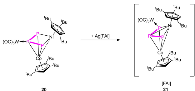
Scheme 5. Oxidation of 20 with Ag[FAl] in CH 2 Cl 2 .
