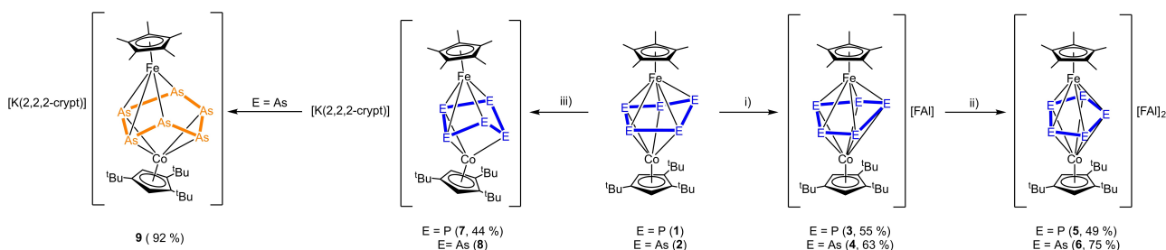
Scheme 2. Reaction of [(\text{Cp}^*\text{Fe})(\text{Cp}'''\text{Co})(\mu, \eta^5: \eta^4\text{-E}_5)] ( \text{E} = \text{P} (1), As (2)) with: i) \text{Ag}[\text{FAl}] in \text{CH}_2\text{Cl}_2 at room temperature; ii) \text{Ag}[\text{FAl}] in o\text{-C}_6\text{H}_4\text{F}_2 at room temperature and iii) \text{K}_8 in the presence of 2,2,2-cryptand in dme.
