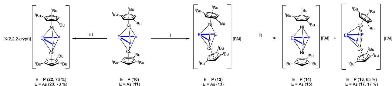
Scheme 3. Reaction of [(Cp''Co)(Cp''Ni)(\mu, \eta^3: \eta^3-E_3)] (E = P (10), As (11) with i) Ag[FAl] in CH_2Cl_2 , ii) leaving the reaction mixture at room temperature overnight and iii) potassium graphite in dme in the presence of 2,2,2-cryptand.
