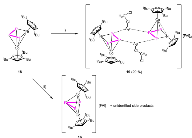
Scheme 4. Reaction of 18 with: i) Ag[FAl] and ii) [Cu(MeCN) 3 ][FAl] in CH 2 Cl 2 at room temperature.
