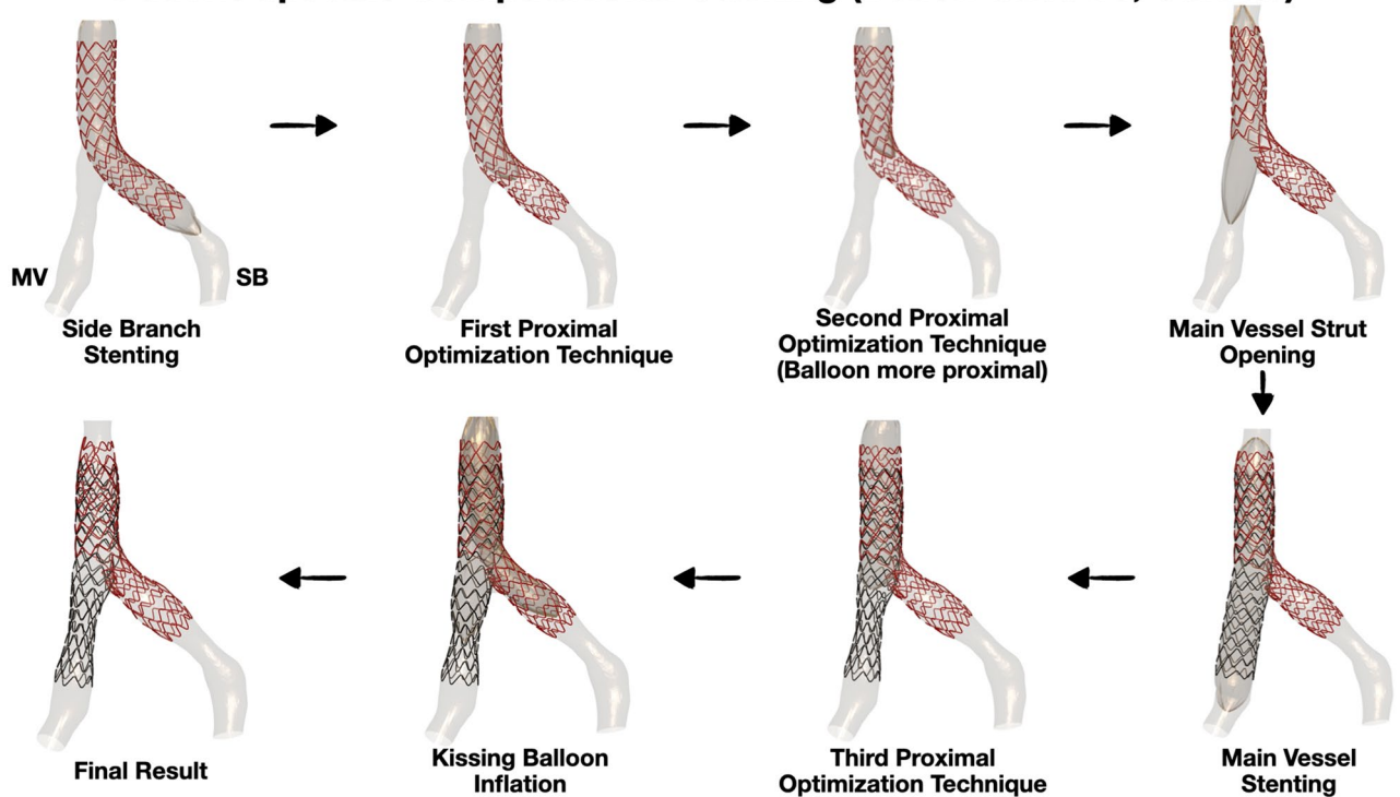
Figure 2. Representative computational simulation of a bench stenting case. A patient-specific silicone bifurcation geometry was stented on the bench with the culotte technique. We faithfully replicated computationally all the steps of the stenting procedure using the same bifurcation geometry and stent/balloon designs; SB side branch, MV main vessel.
