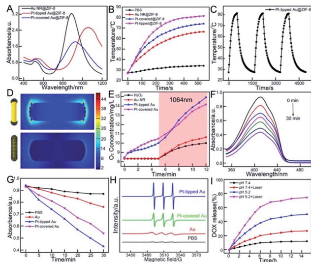
Fig. 2 (A) UV-vis-NIR absorption spectra of Au NR@ZIF-8, Pt-tipped Au@ZIF-8 and Pt-covered Au@ZIF-8. (B) Temperature–time curves of different nanomaterials ( 100 \mu\text{g mL}^{-1} ) under 1064 nm laser irradiation ( 1 \text{ W cm}^{-2} ). (C) The photothermal stability of the Pt-tipped Au@ZIF-8 for three successive cycles of on/off laser irradiation. (D) Electric field enhancement distributions at LSPR excitation based on FDTD simulation. (E) The O_2 concentration of H_2O_2 incubated with different nanoparticles under 1064 nm laser irradiation from the 5th min to the 12th min. (F) Time dependent decrease in the UV-vis absorption spectra of DPBF treated with Pt-tipped Au NRs. (G) Decay curves of DPBF absorption at 410 nm with different nanoparticles. (H) ESR spectra of TEMP/ O_2 adducts collected from H_2O_2 incubated with different nanoparticles. (I) DOX release profiles from DOX-Pt-tipped Au@ZIF-8 complexes with and without NIR laser irradiation at different pH values.
