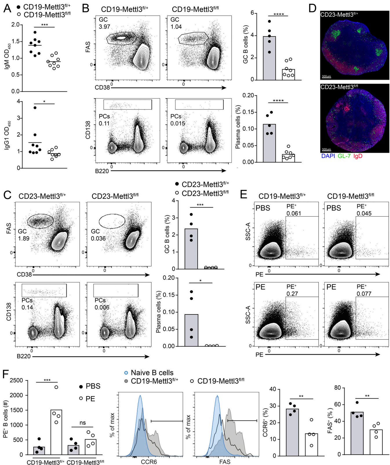
Figure 1. Mettl3 -deficient B cells do not form GCs. (A) Serum Ig titers of IgM and IgG1 in unmanipulated CD19-Mettl3 fl/+ or CD19-Mettl3 fl/fl mice. 8–10 mice per condition, Student's paired t test between age-matched mice was used to determine significance. Lines represent the mean. (B and C) The frequency of GC B cells and PCs in control, CD19-Mettl3 fl/fl (B), or CD23-Mettl3 fl/fl (C) mice, 7 d after NP-KLH immunization. Each data point represents a single mouse, and each column represents the mean value. Pooled data from three experiments with four to seven mice per experiment. (D) Representative immunostained slides of popliteal LNs derived from control or CD23-Mettl3 fl/fl mice. (E and F) Frequency and activation marker expression of naive PE-specific B cells in CD19-Mettl3 fl/+ or CD19-Mettl3 fl/fl 3 d after immunization with PE. Each data point represents a single mouse, and each column indicates the mean value. Pooled data from two experiments each with two mice per condition. SSC, side scatter. *, P < 0.05; **, P < 0.01; ***, P < 0.005; ****, P < 0.001; two-tailed Student's t test (A–E) or one-way ANOVA corrected for multiple comparisons (Sidak; F).
