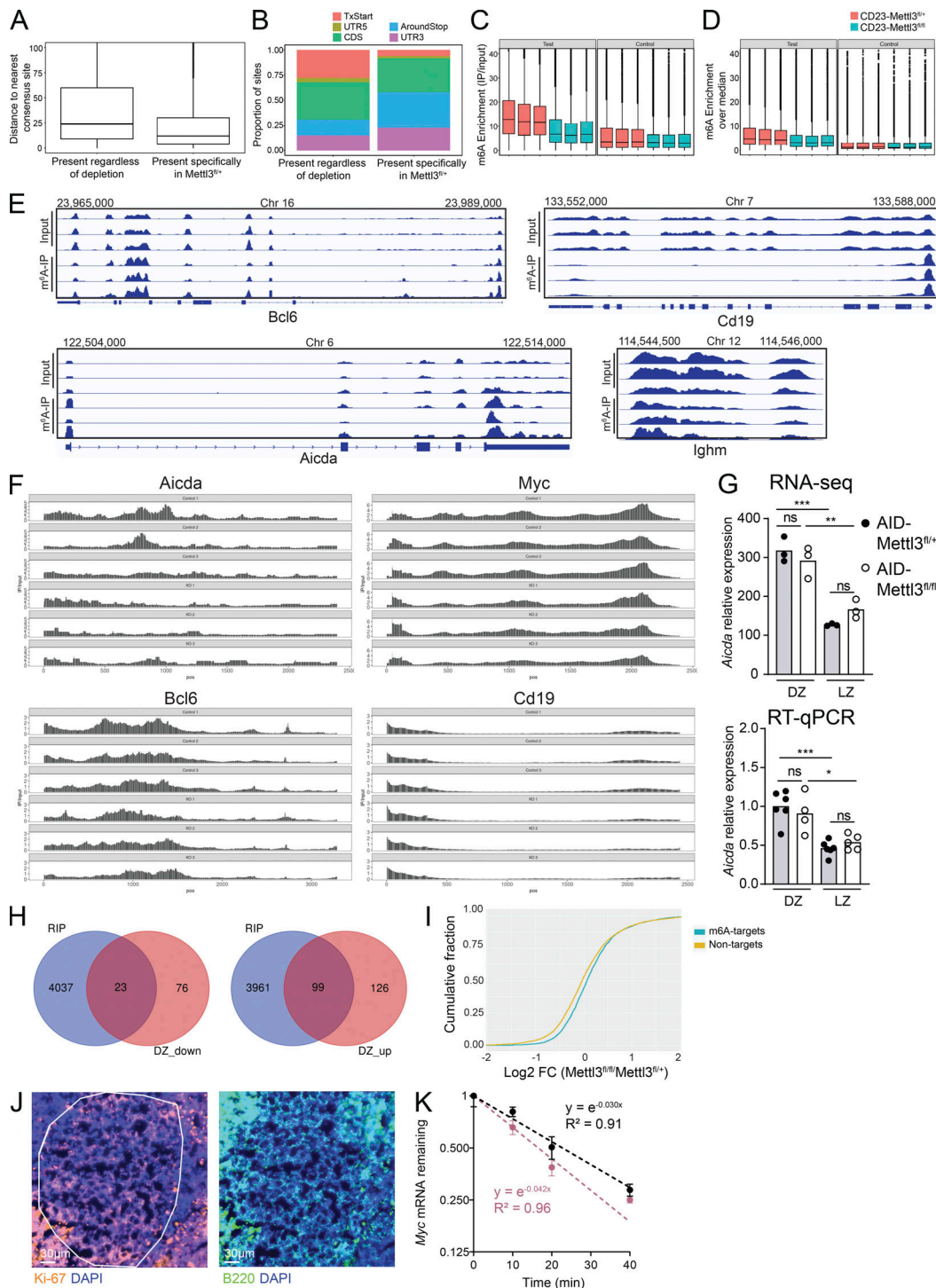
Figure S5. B cells derived from Mettl3 -deficient mice show decreased levels of m 6 A methylation. (A) Analysis of m 6 A abundance in B cells that were stimulated with LPS in vitro. Distributions of distance from the nearest consensus site, of sites that are present only in control samples, or both control and Mettl3 -deficient B cells. (B) Distribution of the sites in A grouped across five gene segments as defined in Dominissini et al. (2012). (C and D) Calculated POI (C) and POM (D) scores for control and Mettl3 -deficient B cells. (E and F) Examples of m 6 A methylation sites in B cell-related genes. Input and m 6 A results are shown separately (E) or as a ratio of IP/Input for control and CD23- Mettl3 fl/fl B cells (F). (G) Aicda mRNA expression as measured by MARS-seq (top) and RT-qPCR (bottom) in GC B cells sorted from immunized control and AID- Mettl3 fl/fl mice 14 d after immunization. Pooled data from two experiments with a total of three to six mice per group. Statistical significance determined using one-way ANOVA with Holm-Sidak's multiple comparisons test. (H) Venn diagrams showing the overlap between m 6 A targets (in LPS-stimulated B cells) and significantly differentially expressed genes (between AID- Mettl3 fl/fl and AID- Mettl3 fl/fl DZ B cells) day 14 after immunization. RIP, RNA immunoprecipitation. (I) Cumulative frequency of mRNA log 2 fold-change (FC) in nontarget and m 6 A-IP target genes upon Mettl3 deletion in DZ GC B cells. (J) Additional supporting results from experiments shown in Fig. 7, C–E. Identification of GC B cells by staining for Ki-67 mRNA (smFISH) and B220 (antibody labeling). (K) Myc mRNA stability assay in B cells isolated from WT and Igf2bp3 -/- mice. Transcription was stopped using actinomycin D, and Myc mRNA levels were measured at increasing time points by RT-qPCR. *, P < 0.05; **, P < 0.01; ***, P < 0.005.
