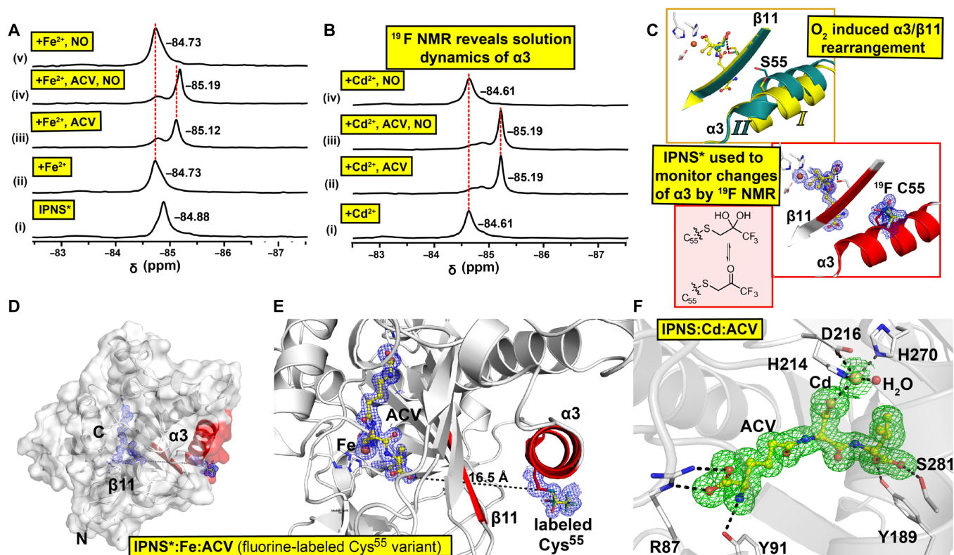
Fig. 7. Spectroscopic analyses in solution support structural dynamics as a consequence of O 2 binding. (A) 19 F NMR spectra from anaerobic solutions of IPNS* ± Fe 2+ ± ACV ± NO support \alpha 3 dynamics after NO binding. (i) IPNS* ( 19 F-labeled IPNS); (ii) IPNS* + Fe 2+ ; (iii) IPNS* + Fe 2+ + ACV; (iv) IPNS* + Fe 2+ + ACV + NO; and (v) IPNS* + Fe 2+ + NO. (B) 19 F NMR of IPNS* ± Cd 2+ ± ACV ± NO. (i) IPNS* + Cd 2+ ; (ii) IPNS* + Cd 2+ + ACV; (iii) IPNS* + Cd 2+ + ACV + NO; and (iv) IPNS* + Cd 2+ + NO (fig. S8). (C) Comparison of the structural elements of \alpha 3/\beta 11 in IPNS:Fe:ACV:O 2 (PDB: 6ZAP) and IPNS*:Fe:ACV (cryo-cooled single-crystal analysis, PDB: 6ZAM, 1.55-Å resolution, used for 19 F NMR, showing keto and gem diol forms of fluorine label). (D) Overview of the IPNS* complex with \alpha 3 and \beta 11 in red and presence of the fluorine label on \alpha 3 . (E) View of the active site and \alpha 3 of the IPNS*:Fe:ACV complex, showing the distance from the ACV valinyl carboxylate to the alkylated Cys 55 (16.5 Å). Changes in the ACV valinyl carboxylate conformation as a function of O 2 binding are proposed to induce structural rearrangement of \alpha 3/\beta 11 . Cys 55 was alkylated with a CH 2 COCF 3 group to study conformational changes in solution by 19 F NMR. Tryptic digestion confirmed the presence of alkylated Cys 55 (fig. S10). (F) Views of the active site of the aerobically grown IPNS:Cd:ACV complex (PDB: 6ZW8, 1.22-Å resolution) obtained by single-crystal cryogenic data collection. A Polder omit map of the active site of IPNS:Cd:ACV after omitting Cd and ACV (3.0 \sigma contour level, green, modeled occupancy of 90% for Cd). Unmodeled electron density was observed next to Trp 213 on the protein surface. Note that exposure of IPNS:Cd:ACV crystals to NO reveals no NO binding to the metal and no evidence for \alpha 3/\beta 11 rearrangements, even after multiple NO exposures with 10 crystals, consistent with the NMR analysis (B).
