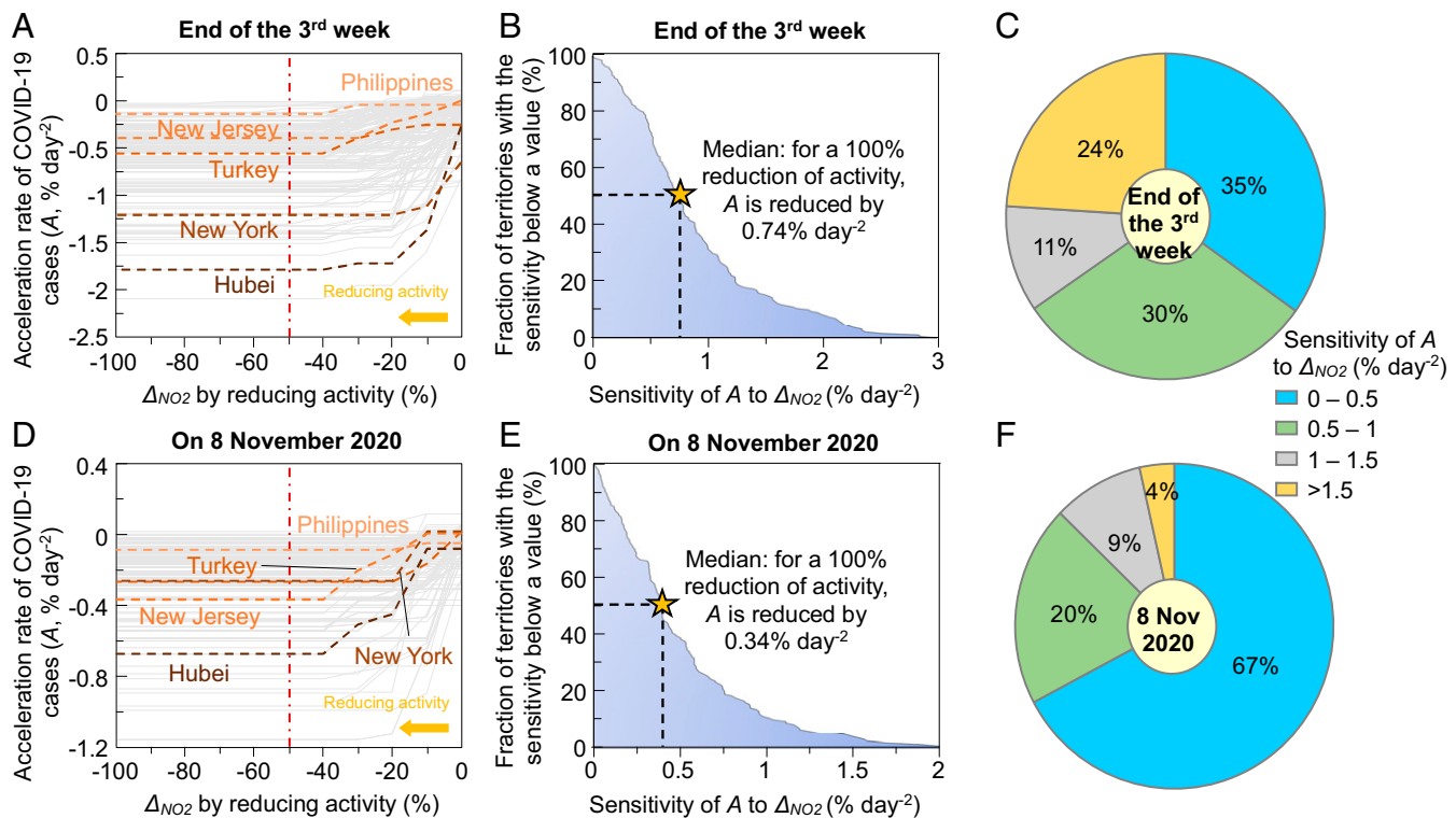
Fig. 5. Global effect of limiting activity in confinement to contain COVID-19. (A) Potential to decelerate the growth of cases ( A ) by reducing \Delta\text{NO}_2 from 0 to -100\% as an indicator for activity reduction at the end of the third week after the COVID-19 outbreak in each territory. (B) Percentages of territories with the sensitivity of A to a reduction of \Delta\text{NO}_2 from 0 to -50\% below a threshold at the end of the third week. (C) Distribution of the A - \Delta\text{NO}_2 sensitivity at the end of the third week. (D–F) As in A–C, except for showing the A - \Delta\text{NO}_2 sensitivity on the last day of \text{NO}_2 observations (8 November 2020) in this study when vaccines had not been widely applied.
