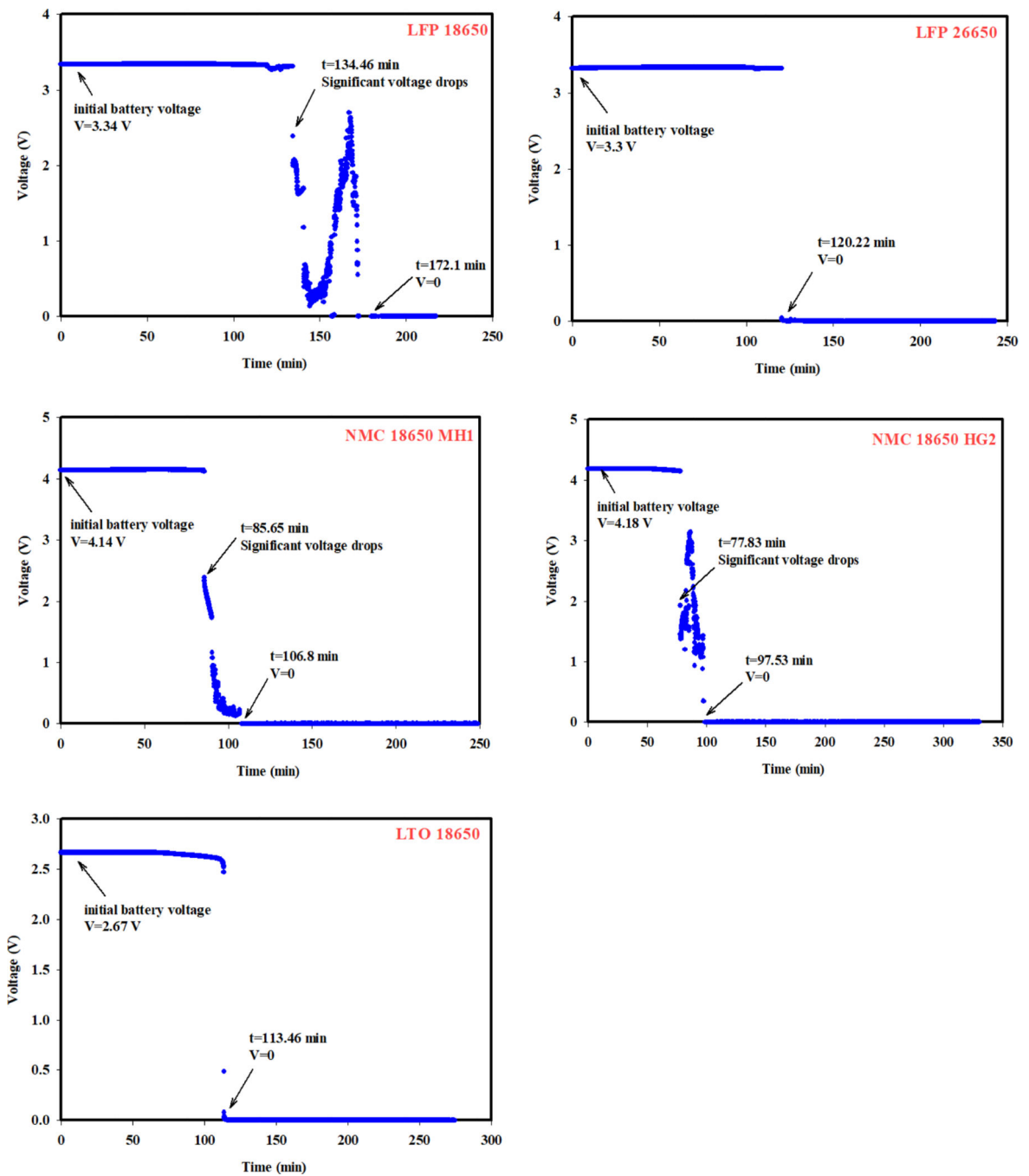
Figure 2. Battery voltage changes in thermal tests
