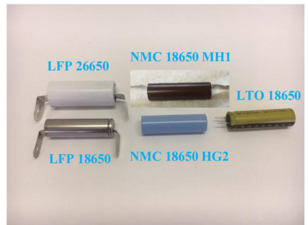
1d. Li-ion cells tested
