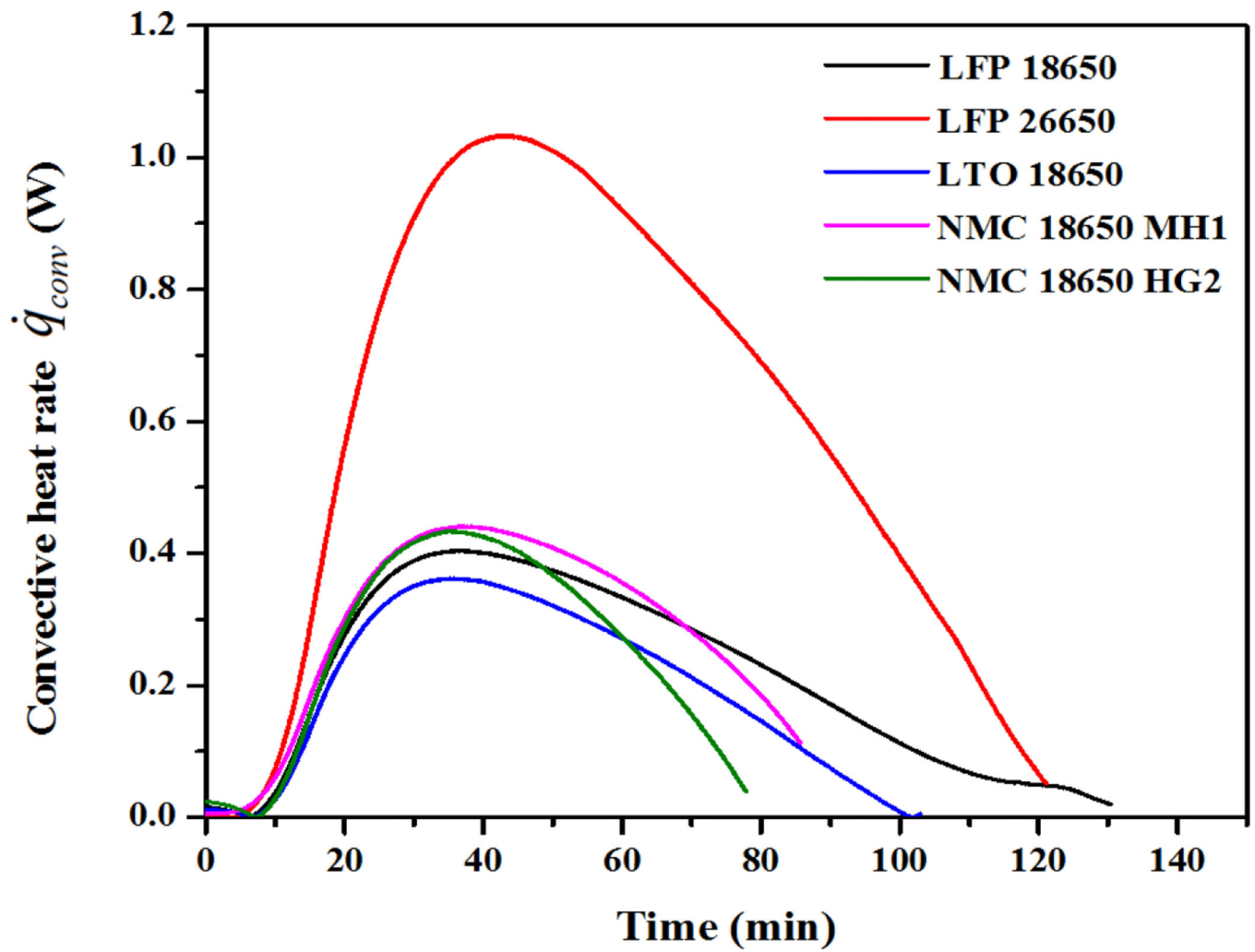
Figure 6. Convective heat transfer to the battery surface
