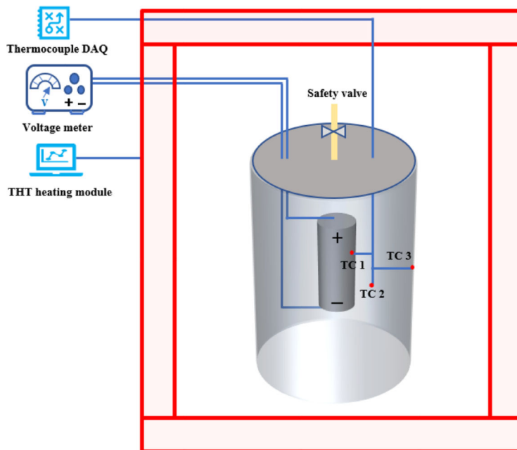
1a. ARC in the battery test lab
