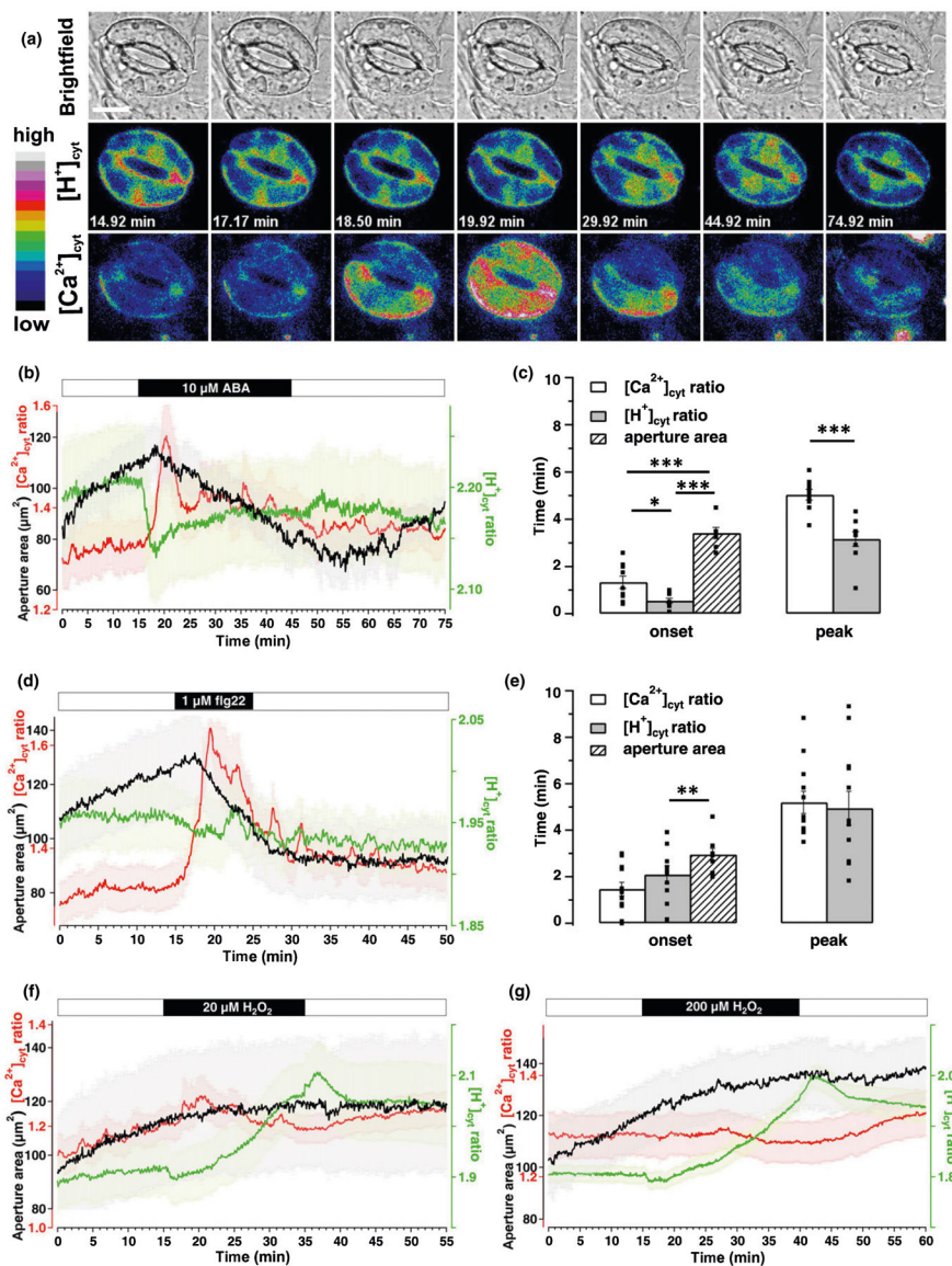
Fig. 4. Different stimuli trigger distinct [\text{Ca}^{2+}]_{\text{cyt}} and [\text{H}^+]_{\text{cyt}} signatures in guard cells (GCs) during stomata movement. Time-lapse CapHensor imaging together with stomata aperture monitoring in GCs of Nicotiana tabacum epidermal strips. (a) Brightfield (top) as well as false colored [\text{H}^+]_{\text{cyt}} (middle) and [\text{Ca}^{2+}]_{\text{cyt}} (bottom) ratio images of a representative time-lapse CapHensor imaging series upon the application of 10 \mu\text{M} ABA. Bar, 20 \mu\text{m} . (b, d, f, g) Mean [\text{Ca}^{2+}]_{\text{cyt}} ratio (red), [\text{H}^+]_{\text{cyt}} ratio (green) and stomatal aperture area (black) over time upon application of (b) 10 \mu\text{M} ABA ( n = 10 ), (d) 1 \mu\text{M} flg22 ( n = 12 ), (f) 20 \mu\text{M} \text{H}_2\text{O}_2 ( n = 10 ) and (g) 200 \mu\text{M} \text{H}_2\text{O}_2 ( n = 22 ). The bars above the mean traces indicate the time of treatments. (c, e) Bar diagram displays the average time of the onset and to the peak-response after 10 \mu\text{M} ABA and 1 \mu\text{M} flg22 treatment from data shown in (b) and (d), respectively. Dots in (c) and (e) indicate individual measurements. Error bars = SE.
