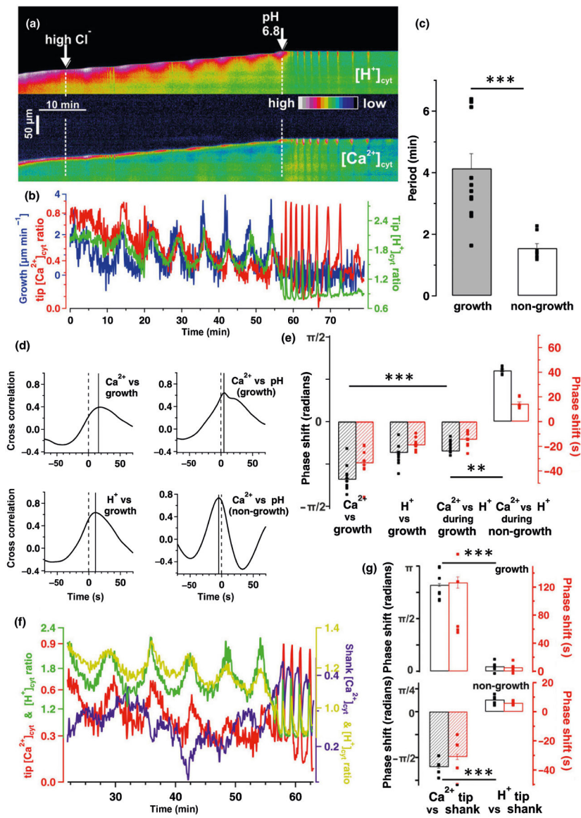
Fig. 3. Phase-relation analyses of [Ca 2+ ] cyt , [H + ] cyt and growth in oscillating pollen tubes (PTs). Live-cell CapHensor imaging of oscillating Nicotiana tabacum PTs to quantify spatio-temporal interrelation of ion signaling and growth. (a) False colored [H + ] cyt -ratio (top) and [Ca 2+ ] cyt -ratio (bottom) kymographs from a representative PT upon external challenging with 20 mM chloride (Cl - ) and later challenged with both 20 mM Cl - and pH 6.8 medium. (b) Quantification of PT tip [Ca 2+ ] cyt (red line), [H + ] cyt (green line) and growth rate (blue line) of the experiment in (a). (c) Mean period of [Ca 2+ ] cyt - and [H + ] cyt -ratio oscillations in growing (grey, n = 13) and non-growing (white, n = 8) PTs in high Cl - -solution. (d, e) Quantification of phase relationships via (d) cross-correlation and (e) cross-wavelet analyses from growing ( n = 10) and non-growing ( n = 8) PTs in high Cl - -solution as in (b). Time between the solid and dotted vertical lines corresponds to the lagging (shift to right side) or leading (shift to left side) signals in (d). Phase relationship of the signals is presented in
