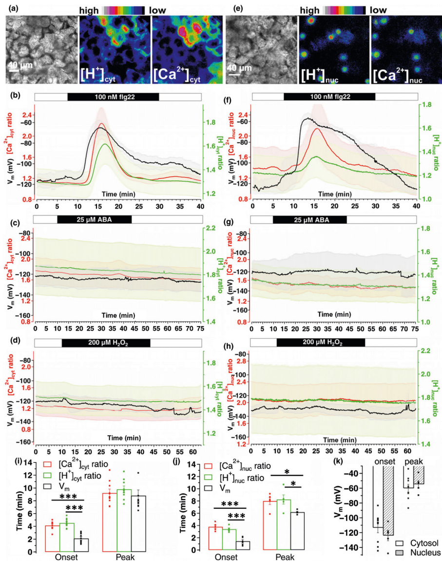
Fig. 6. Distinct cytosolic and nuclear Ca^{2+} - and H^+ -signatures in mesophyll cells upon different stimuli. Simultaneous Ca^{2+} , H^+ and V_m recordings in mesophyll cells of Nicotiana benthamiana leaves transiently expressing a cytosolic or nuclear version of the CapHensor. (a, e) Representative brightfield (left) as well as false colored [H^+] - (middle) and [Ca^{2+}] (right) ratio images of a leaf mesophyll section expressing the (a) cytosolic- or (e) nuclear CapHensor version. (b–d) Mean [Ca^{2+}]_{cyt} ratio (red), [H^+]_{cyt} ratio (green) and membrane potential ( V_m , black) dynamics over time upon application of (b) 100 nM flg22 ( n = 9 ), (c) 25 \mu M ABA ( n = 6 ) and (d) 200 \mu M H_2O_2 ( n = 5 ). (f–h) Mean [Ca^{2+}]_{nuc} ratio (red), [H^+]_{nuc} ratio (green) and V_m (black) dynamics over time upon application of (f) 100 nM flg22 ( n = 6 ), (g) 25 \mu M ABA ( n = 4 ) and (h) 200 \mu M H_2O_2 ( n = 5 ). (i, j) Bar diagram of mean onset and peak times of Ca^{2+} ratio (red), H^+ ratio (green) and V_m after 100 nM flg22 with the cytosolic (i) or nuclear (j) expressed CapHensor. (k) Bar diagram of mean membrane
