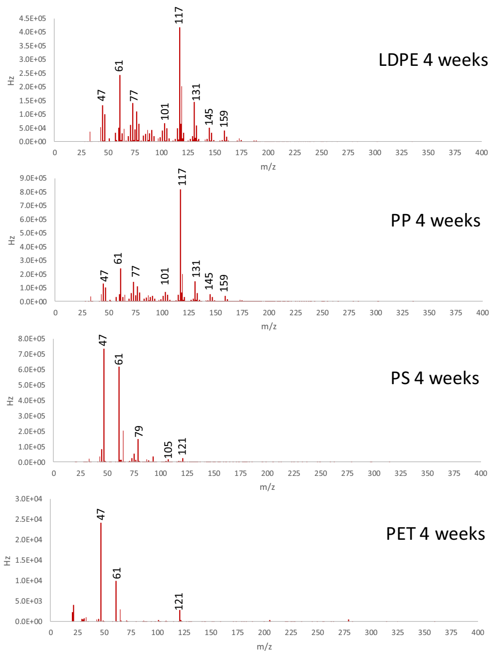
Fig. 10 Artificially aged MPs: SIFT-MS mass spectra obtained with [H_3O]^+ reactive ion
