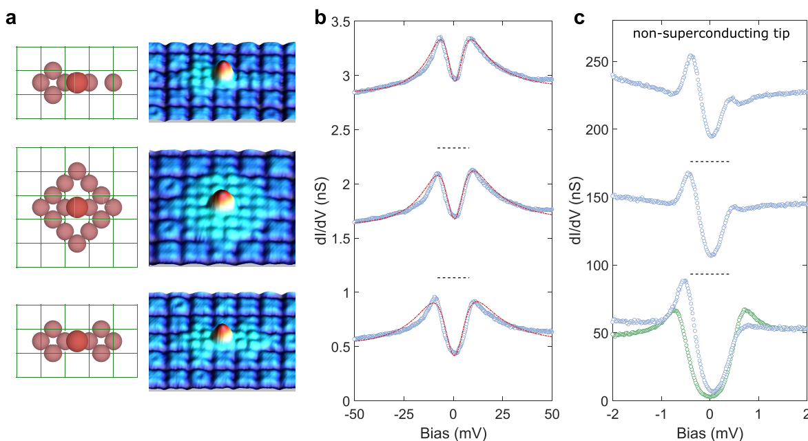
Figure 2. Construction and spectroscopy of large Fe clusters. (a) Schematic top-view and the corresponding STM images of an Fe adatom with assemblies of a large number of IFAs ( V = 50 mV, I = 50 pA). (b) Large-bias dI/dV spectra (open dots) measured with W tip showing the split Kondo resonance. The dashed red lines are fits to a Fano function, which is multiplied by a Lorentzian dip. Spectra are shifted vertically for clarity as indicated by the dashed horizontal zero lines. Stabilization parameters for STS are V_{\text{stab}} = 50 mV, I_{\text{stab}} = 100 pA, V_{\text{mod}} = 2 mV. (c) Corresponding small-bias dI/dV spectra showing peaks inside the superconducting gap due to YSR states, plotted together with substrate spectrum. Spectra are shifted vertically for clarity as indicated by the dashed horizontal zero lines. Stabilization parameters for STS are V_{\text{stab}} = 4 mV, I_{\text{stab}} = 200 pA, V_{\text{mod}} = 50 \mu V.
