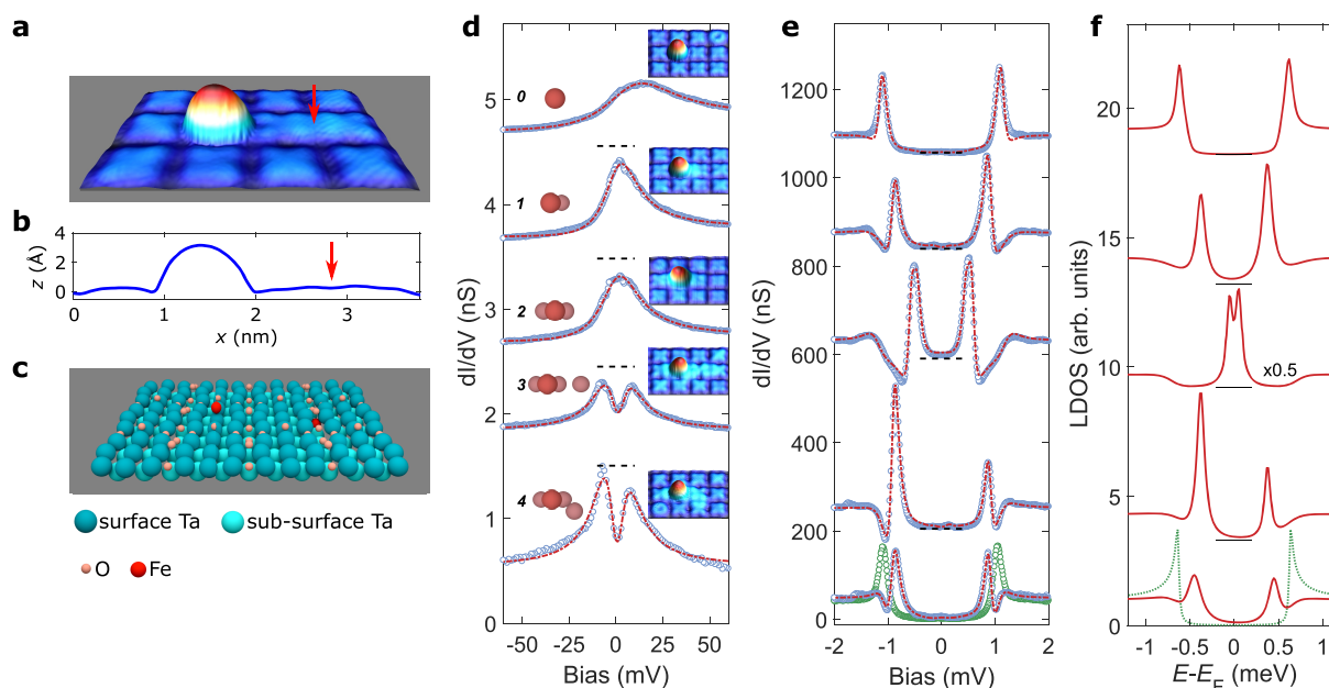
Figure 1. Construction and spectroscopy of Fe clusters at the TaO surface. (a) Constant-current STM image of the TaO surface with an Fe adatom and an interstitial Fe atom (IFA) indicated by the red arrow. (b) Height profile across the IFA and the Fe adatom in (a). (c) Perspective view of the DFT-optimized fully relaxed positions of an Fe adatom, an IFA, and the atoms in the TaO surface. (d) Large-bias dI/dV spectra showing the Kondo resonance. The dashed red lines are fits to a Fano function, which is multiplied by a Lorentzian dip for the spectra exhibiting the zero-bias anomaly (ZBA), i.e., the exchange splitting of the Kondo resonance (see Supporting Information). The pictograms and numbers on the left side of the spectra show the corresponding structure of the Fe clusters and numbers of the IFAs in the assemblies. Corresponding STM images are shown in the insets on the right side of the curves ( V = 50 mV, I = 100 pA). Spectra are shifted vertically for clarity as indicated by the horizontal dashed zero lines. Stabilization parameters for STS are V_{\text{stab}} = 100 mV, I_{\text{stab}} = 100 pA, V_{\text{mod}} = 2\text{--}4 mV. (e) Small-bias dI/dV spectra (open dots) showing peaks inside the superconducting gap due to YSR states, together with the substrate spectrum (open green dots). Dashed red lines are fits obtained using a numerical deconvolution method. Spectra are shifted vertically for clarity as indicated by the horizontal dashed zero lines. Stabilization parameters for STS are V_{\text{stab}} = 2.5 mV, I_{\text{stab}} = 100 pA, V_{\text{mod}} = 20 \mu V. The corresponding deconvoluted LDOS is plotted in (f). The green curve in (f) corresponds to the reference substrate density of states.
