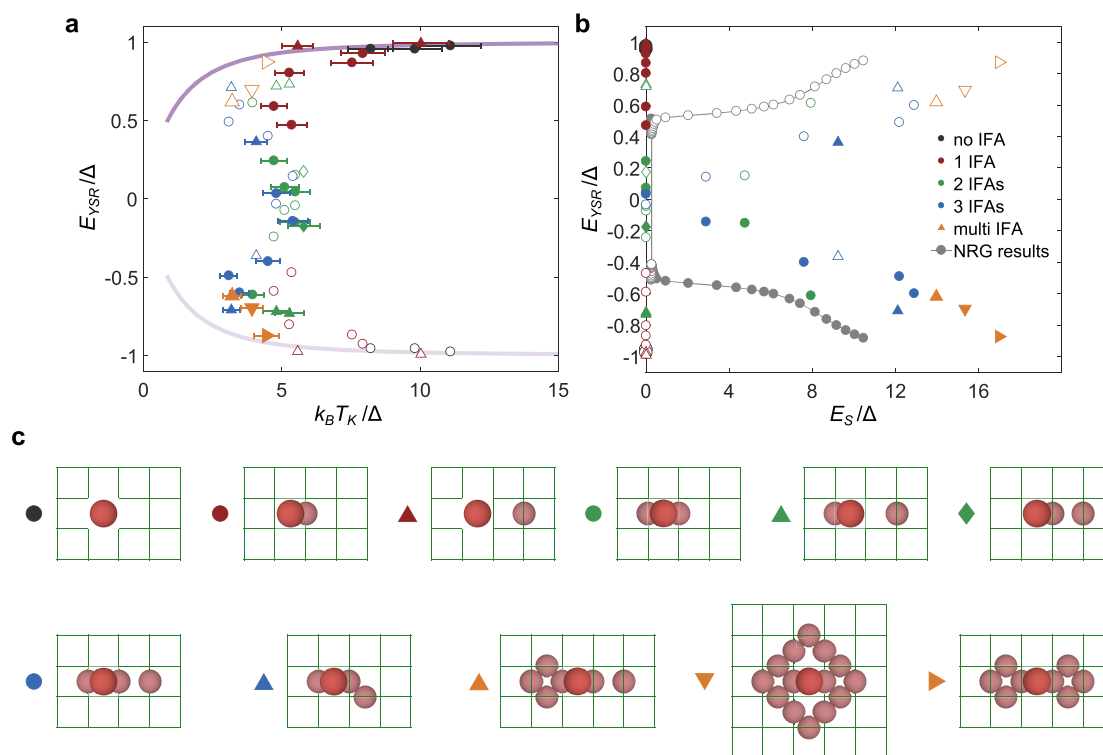
Figure 3. Correlation of Kondo temperature, exchange splitting, and YSR state energy. (a) Scatter plot of the energy of the larger YSR peak (filled symbols) versus the Kondo temperature, both extracted from the experimentally investigated Fe adatom with different IFA assemblies. The open symbols give the sign-reversed values of the energies of the corresponding filled symbols. Various types of symbols in the plot represent various types of IFA assemblies as indicated in (c). Horizontal error bars indicate the estimated errors in the fitting of the Kondo-resonance width. The violet curve in (a) represents the slave-boson mean-field theory calculation. (b) Scatter plot of the energy of the larger YSR peak (filled symbols) and its sign-reversed values (open symbols) versus the exchange splitting of the Kondo resonance, both extracted from the experimentally investigated Fe adatom with different IFA assemblies (assignment of the symbols to the different assemblies, see (c)). Results of the NRG calculations, which are plotted as filled and open gray dots, show qualitative agreement with the experiments. All energy scales are normalized to the energy gap ( \Delta ) of the superconducting substrate.
