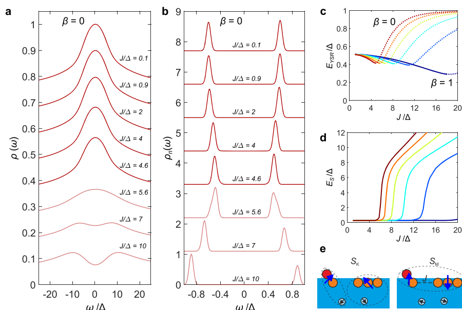
Figure 4. Numerical renormalization group calculations. (a) Spectral function of the impurity representing the pair of adatom and closest IFA (see (e)), which is magnetically coupled to a second impurity representing the rest of the IFA assembly, on the energy scale of the Kondo peak for various magnetic interaction strengths J . The superconducting gap is washed out here using a convolution which mimics the experimental lock-in-modulation broadening. The line style indicates the nature of the ground state of the system (solid lines as Kondo vs dotted lines as AFM) controlled by the strength of J . (b) Discrete (subgap) part of the spectral function. A narrow Gaussian kernel is used to broaden the \delta peaks. For (a) and (b), the isotropic Heisenberg limit of the model \beta = 0 has been assumed. (c) Energy of the YSR state as a function of J . (d) Width of the exchange-splitting gap as a function of J . For (c) and (d) the line colors represent different values of \beta which range from 0 (red, isotropic Heisenberg limit) to 1 (dark blue, anisotropic Ising limit) in steps of 0.2. (e) Schematic illustration of the minimal two-impurity Kondo problem. The Fe (red sphere)/proximal IFA (orange sphere) pair is represented by the first effective spin-1/2 impurity (left blue arrow), and the assembly of additional IFAs (three orange spheres) is represented by the second effective spin-1/2 impurity (right blue arrow). Both impurities Kondo-couple to substrate electrons (smaller spheres). The left and right panels illustrate the two regimes of decoupled Kondo singlets ( S_K , small J ) and AFM singlet ( S_M , large J ).
