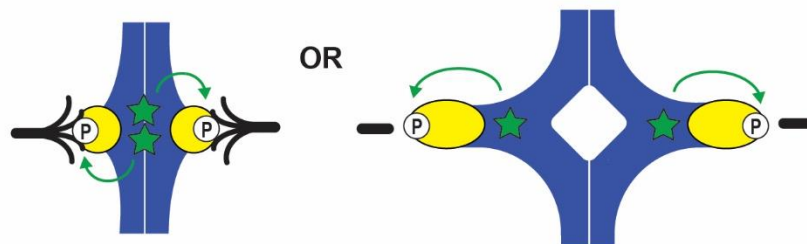
Figure 3. Current models of Aurora-B tension-sensing mechanisms. Chromatids (blue) and bound by kinetochores (yellow) are regulated by Aurora B (star) based on tension. Attachments to microtubules
