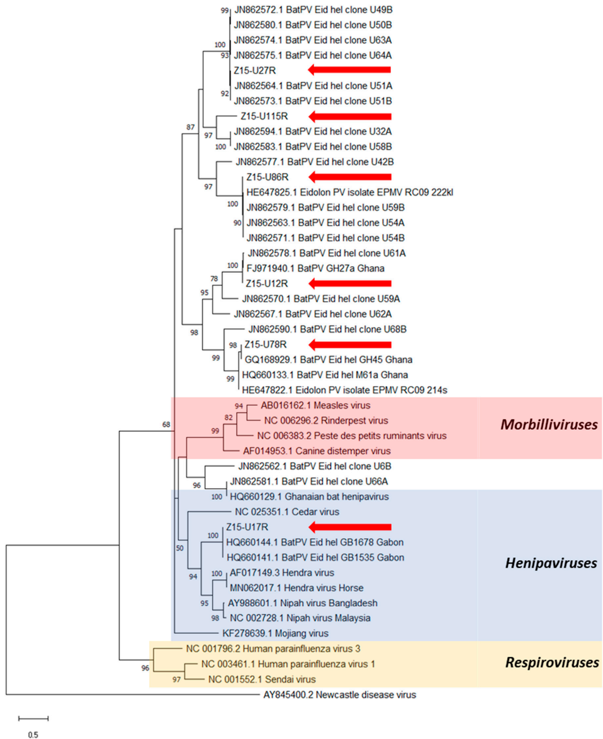
Figure 4. Phylogenetic analysis of partial L gene sequences obtained after RMH-PCR on E. helvum urine samples (red arrows). Maximum likelihood tree with bootstrapping (1000 iterations) generated in MEGA X, using 439 bp alignment against publicly available paramyxovirus sequences (NCBI Genbank) and outgroup Newcastle disease virus. Bootstrap values for 1000 replicates are indicated as percentages (where >50%) and the number of nucleotide substitutions per site is to scale as indicated by the scale bar.
