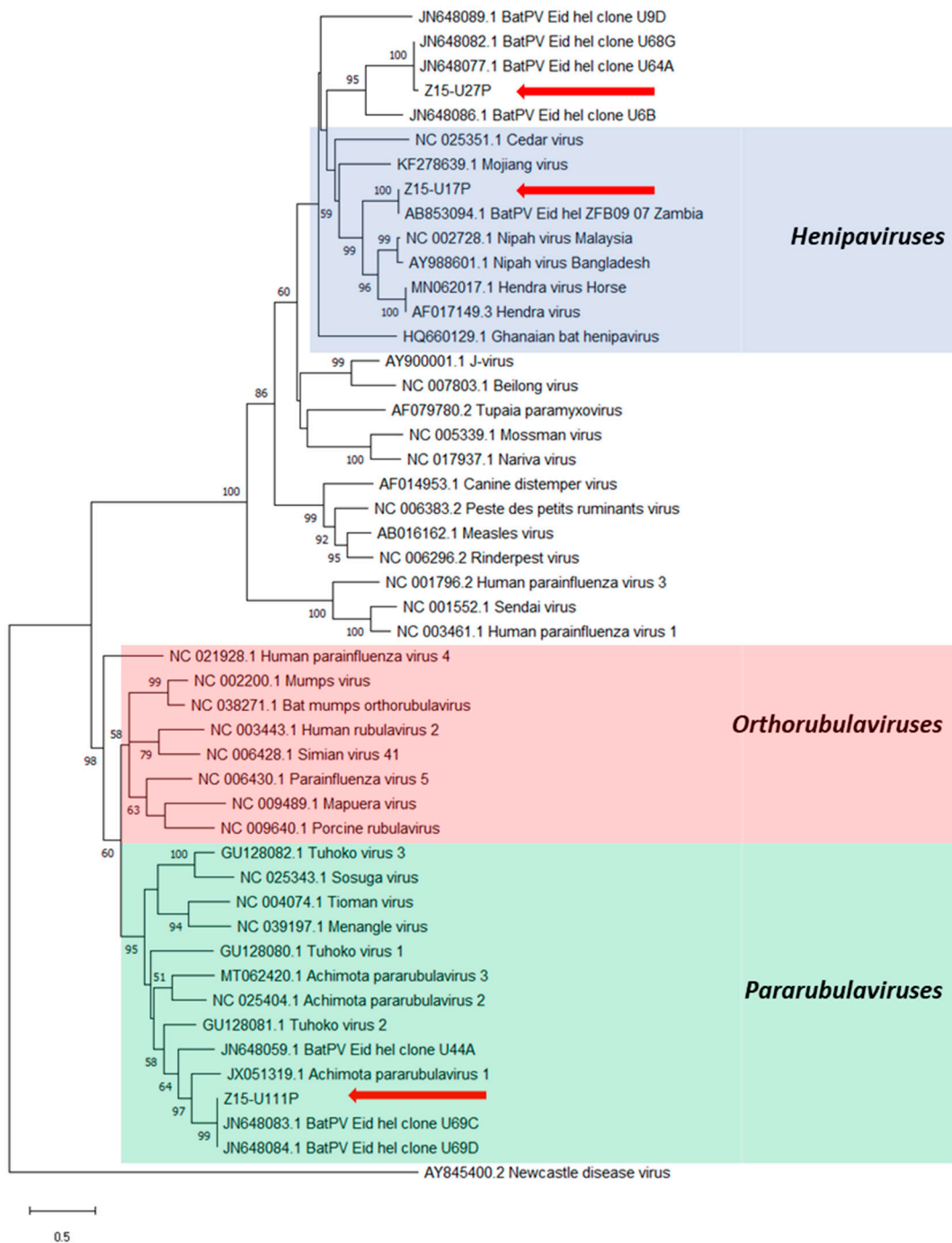
Figure 3. Phylogenetic analysis of partial L gene sequences obtained after PAR-PCR on E. helvum urine samples (red arrows). Maximum likelihood tree with bootstrapping (1000 iterations) generated in MEGA X, using 530 bp alignment against publicly available paramyxovirus sequences (NCBI Genbank) and outgroup Newcastle disease virus. Bootstrap values for 1000 replicates are indicated as percentages (where >50%) and the number of nucleotide substitutions per site is to scale as indicated by the scale bar.
