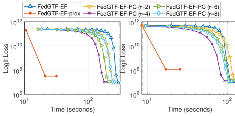
Figure 6: Comparison of different number of workers on 3rd order CMS for Bernoulli Logit Loss.
