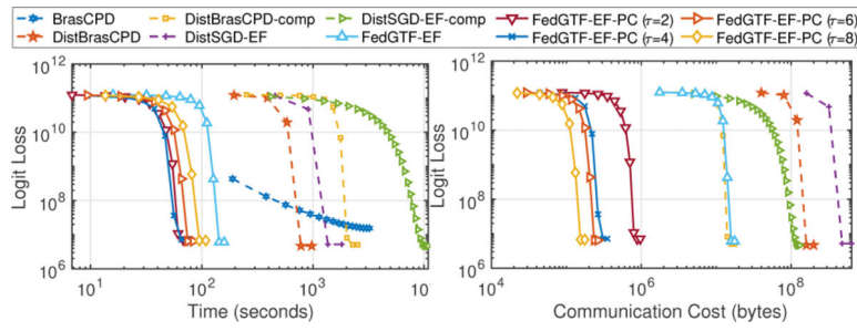
Figure 5: Ablation Study on 3-rd order CMS for Bernoulli Logit Loss.
