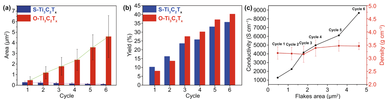
Fig. 3 Comparison of a average flakes area and b yield at different cycles between S- \text{Ti}_3\text{C}_2\text{T}_x and O- \text{Ti}_3\text{C}_2\text{T}_x . c Conductivity (black) and density (red) of O- \text{Ti}_3\text{C}_2\text{T}_x films versus flakes area. Cycle 1 to Cycle 6 in the figure represents the O- \text{Ti}_3\text{C}_2\text{T}_x products corresponding to different cycles
