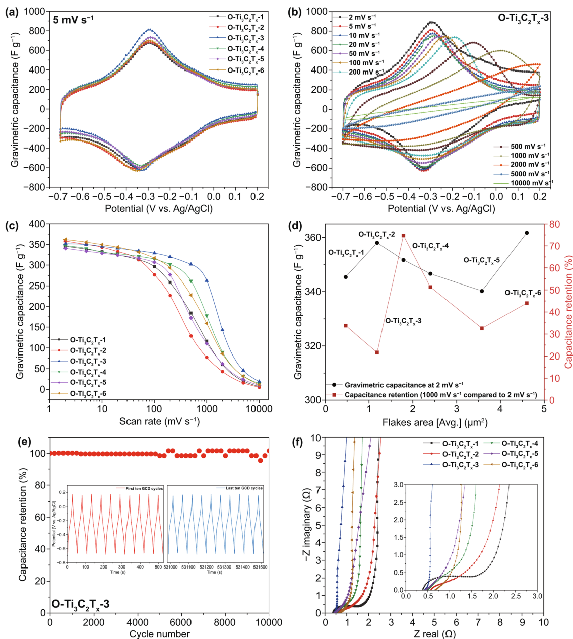
Fig. 5 Electrochemical performance of O-Ti 3 C 2 T x film electrodes. a Cyclic voltammogram profiles collected in 3 M H 2 SO 4 at 5 mV/s scan rate of O-Ti 3 C 2 T x film electrodes from products of different cycles (denote as O-Ti 3 C 2 T x -1 to O-Ti 3 C 2 T x -6). b CV profiles of O-Ti 3 C 2 T x -3 at scan rates from 2 mV s -1 to 10 V s -1 . c Gravimetric capacitance of O-Ti 3 C 2 T x film electrodes at different scan rates d Gravimetric capacitance at scan rate of 2 mV s -1 and rate performance (scan rate at 1000 mV s -1 compared to at 2 mV s -1 ) of O-Ti 3 C 2 T x film electrodes versus different flakes areas. e Capacitance stability of O-Ti 3 C 2 T x -3 performed by GCD cycling at 10 A g -1 . The insets depict GCD cycling profiles collected at first ten cycles (red) and last ten cycles (blue), respectively. f Electrochemical impedance spectroscopy (EIS) for O-Ti 3 C 2 T x film electrodes. The inset shows a magnification of the high-frequency region
