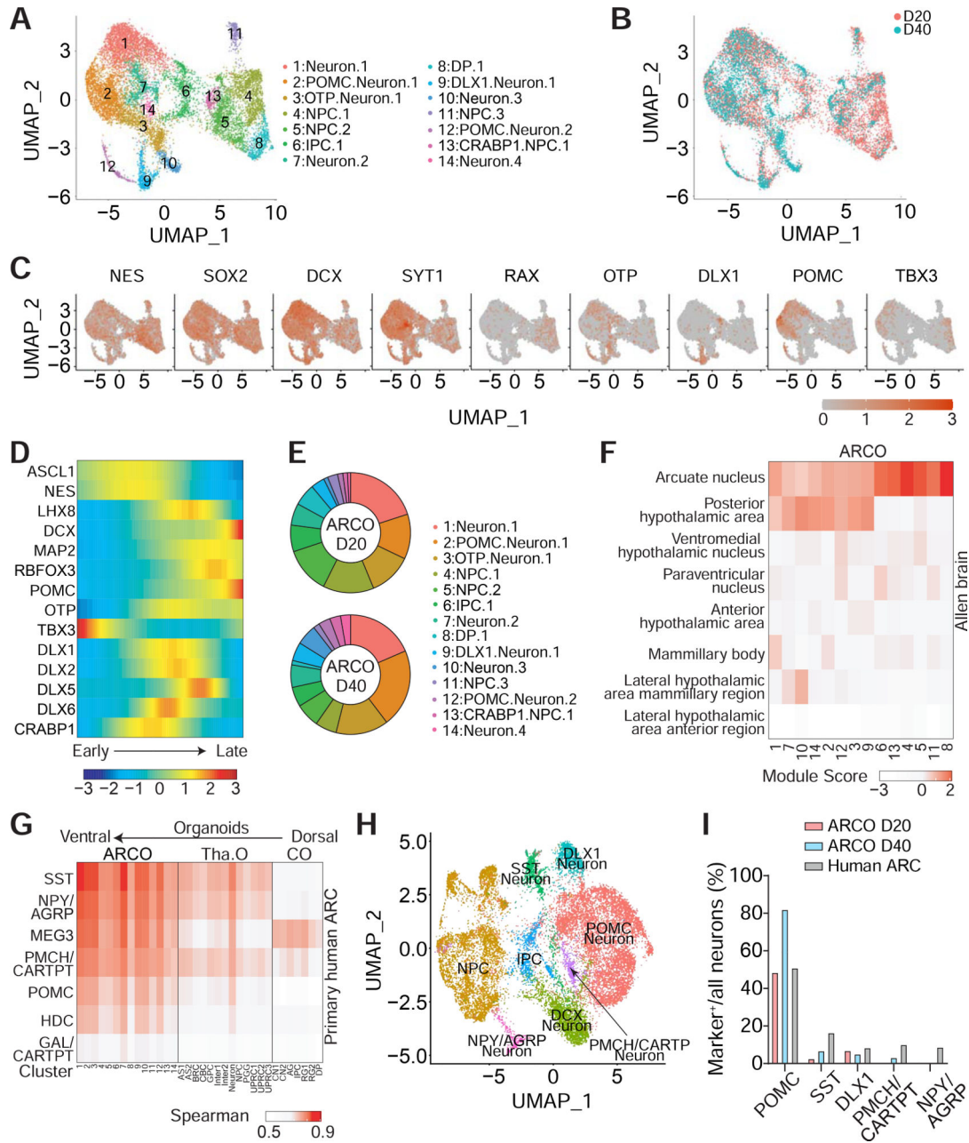
Figure 2. Single-Cell RNA-Seq Analyses of ARCOs.
