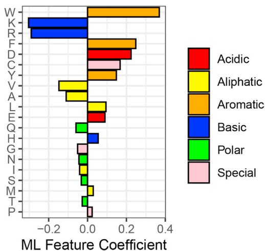
Figure 8. Within the subpool of net-positively charged sequences, Cysteine gains importance for prediction of tAD functionality
