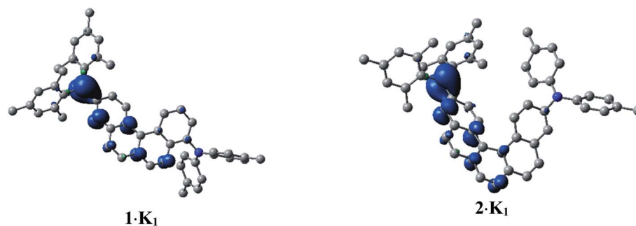
Fig. 7 Spin density plots of 1\cdot\mathbf{K}_1 (doublet) and 2\cdot\mathbf{K}_1 (doublet), calculated as naked 1^{1-} and 2^{1-} species. H-atoms are omitted for clarity. Isovalue: \pm 0.003 [e_a^{-3}]^{1/2} .
